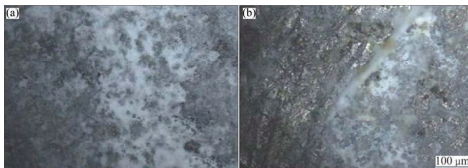
Fig. 20 Optical images of Zn–Al–Sn–Ti–Cl–0.3V (a) and Zn–Al–13Sn–Ti (b) chloride deposited samples after corrosion
