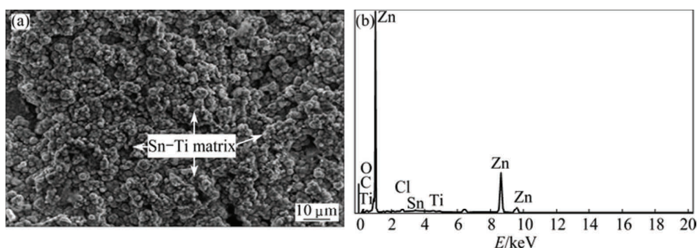
Fig. 4 SEM image (a) and EDS result (b) of Zn-Al-7Sn-Ti-0.3V chloride deposited sample
