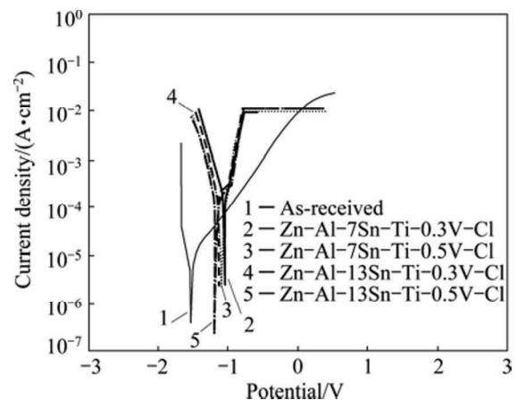
Fig. 18 Potentiodynamic polarization curves for Zn–Al–Sn–Ti chloride deposited
