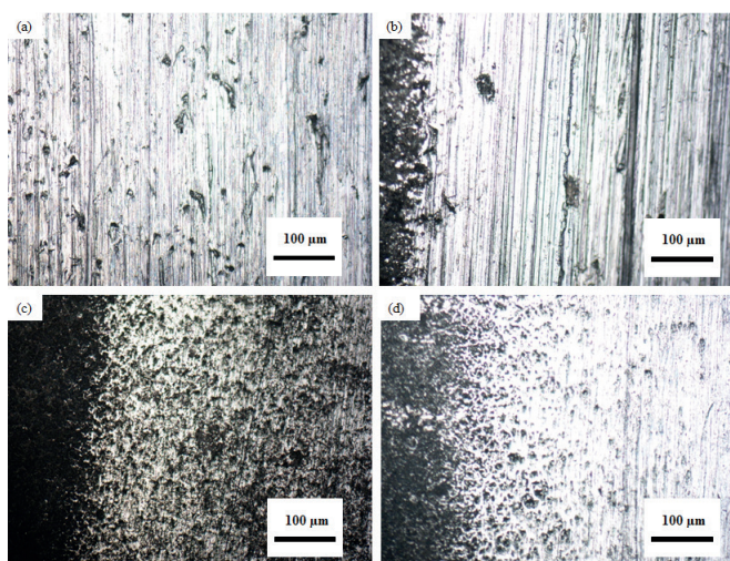
Fig. 11. Optical Microscope micrographs of worn out surfaces (a) as received sample, (b) Zn electrodeposits (c) ZA1 alloy and (d) ZC2 nanocomposite alloy
