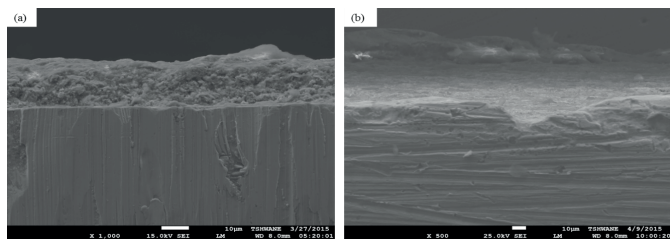
Fig. 3. SEM images of the cross section (a) ZA1 and (b) ZC2 nanocomposite coatings
