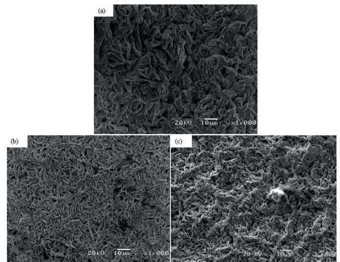
Fig. 2. SEM micrographs (a) Zn coating (b) Zn-5g/L \text{Al}_2\text{O}_3 coating and (c) Zn-20g/L \text{Cr}_2\text{O}_3 coating
