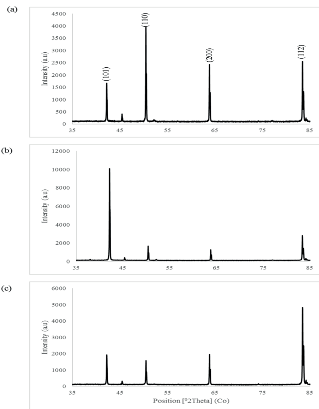
Fig. 5. X-ray diffractograms of (a) Zn coating, (b) ZA1 composite coating and (c) ZC2 composite coating
