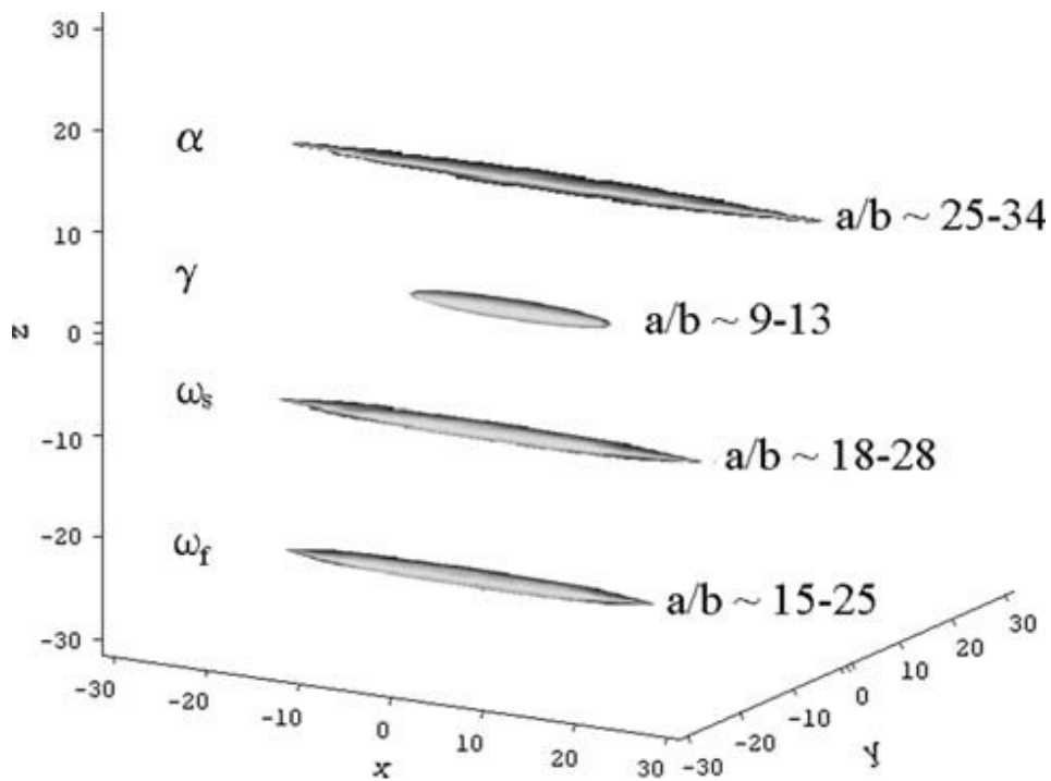
Figure 3 – schematic representation for gliadin fractions: \alpha -gliadin; \gamma -gliadin; \omega_s -gliadin and \omega_f -gliadin in terms of prolate ellipsoids ( x , y and z represent the orthogonal axes in which the ellipsoid lies and a , b and c are ellipsoid semi-axes ( a \geq b \geq c ) in the x , y and z directions with, c = a for an oblate ellipsoid and c = b for a prolate ellipsoid). The axial ratio is shown is median value from Table 2 ( a/b \sim 30, 11, 23 and 20 , respectively).
