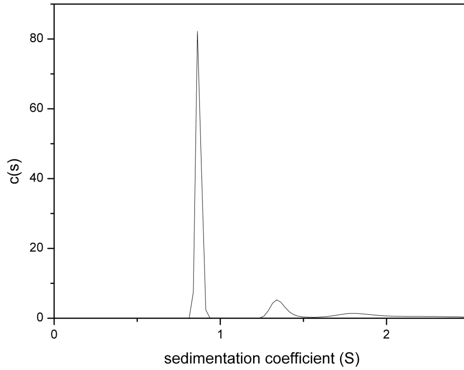
Figure 1 – c(s) profile for whole gliadin at a nominal total loading concentration of 2.0 mg/mL.
