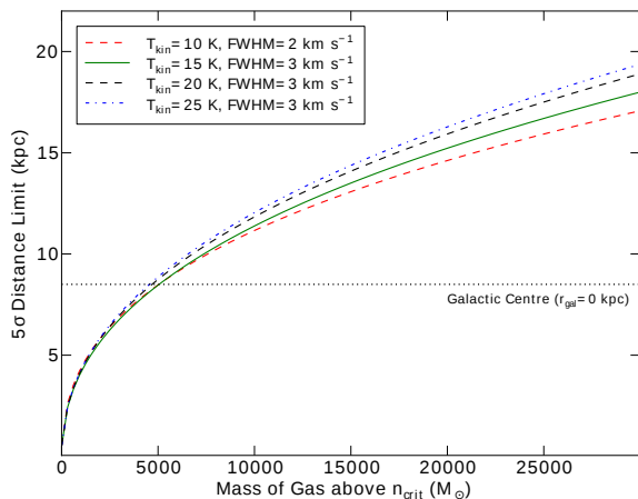
Figure 14. Plot of the 5\sigma detection limit distance versus mass of gas above the \text{NH}_3 critical density ( n_{\text{crit}} \approx 10^4 \text{ cm}^{-3} ) for clouds with representative excitation conditions. The dotted line shows the distance of the Galactic centre at 8.5 kpc.
