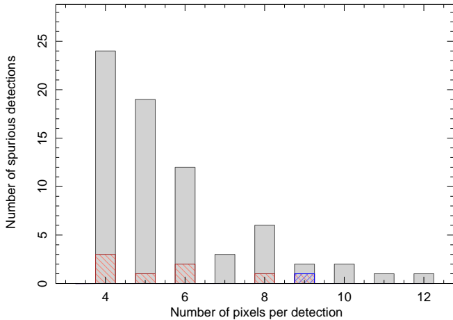
Figure 11. Histogram of the number of spurious sources detected in an ‘empty’ \text{NH}_3 (2,2) data cube (see Section 5.3.1 for details). The source finder was run at a range of sigma-limits to characterise the number of detections as a function of source solid angle. Grey bars = 0.7\sigma , red-hatched (left-slanted) bars = 0.8\sigma and blue-hatched (right-slanted) bars = 0.9\sigma . Based on this plot a brightness cutoff of 0.8\sigma was selected and a minimum of seven spatial pixels was required in a valid detection. The artificially low \sigma -limit is possible because the à trous reconstruction effectively suppresses most of the noise.
