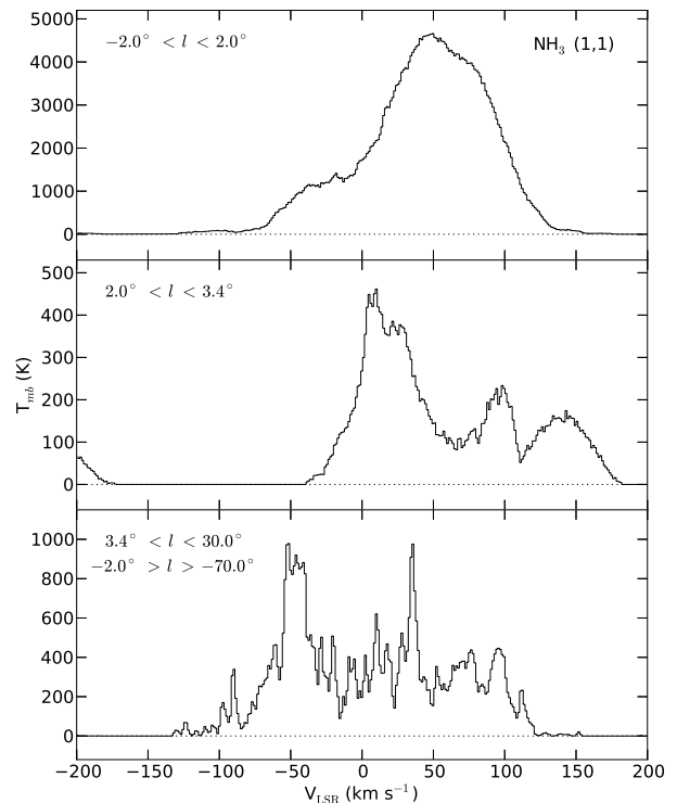
Figure 6. Integrated \text{NH}_3 (1,1) spectrum for the Galactic centre (top panel), the region around the G3.34+0.42 cloud, also known as Bania’s Clump 2 (middle panel), and the outer Galaxy (bottom panel). Spectra were integrated over the full latitude range ( \pm 0.5^\circ ).
