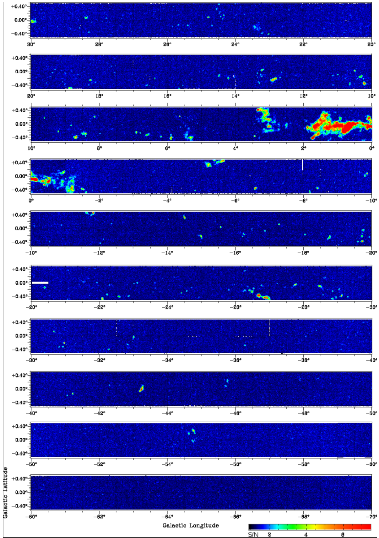
Figure 2. Map of the peak NH 3 (2,2) signal-to-noise (S/N) across the HOPS survey area.
