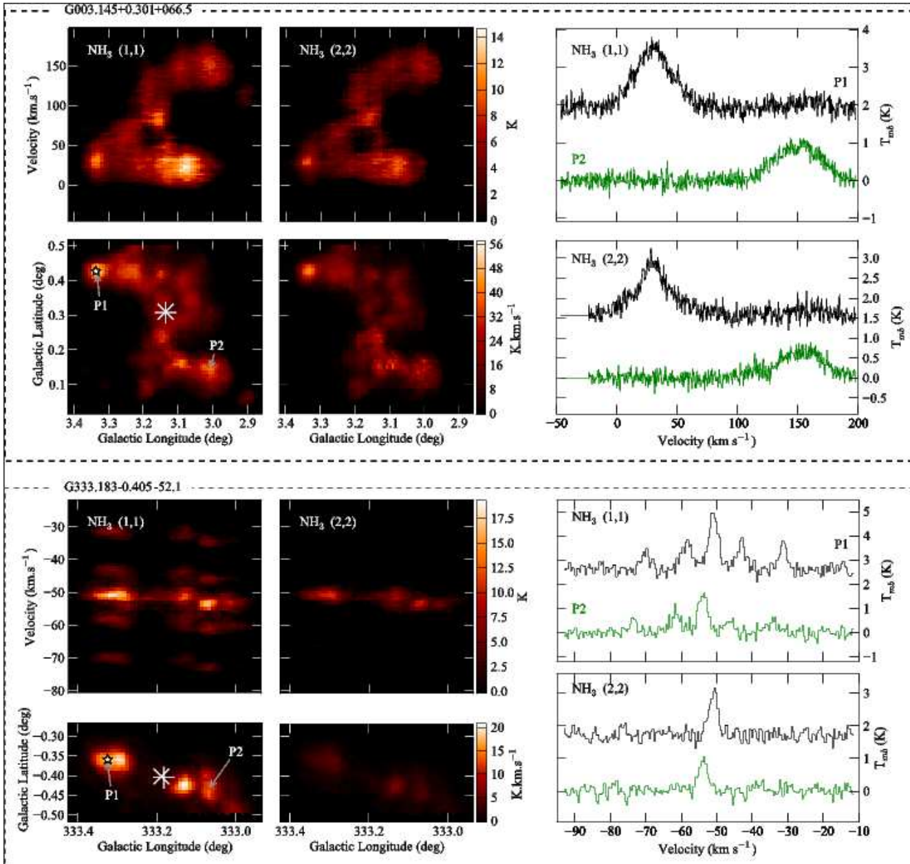
Figure 10. Examples of two bright clouds in HOPS. For each cloud we show the \text{NH}_3 (1,1) and (2,2) integrated intensity maps (bottom-left and bottom-middle panels, respectively), summed longitude velocity ( l - v ) diagrams (top-left and top-middle panels) and sample spectra from two local peak positions (right panels). The l - v diagrams were made by summing over the Galactic b axis of the cubes. The position of the brightest voxel is marked by a star symbol, the geometric centre by a '+' and the brightness-weighted centre by a 'x'. See section 4.3 for details.
