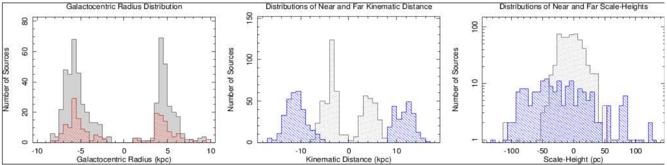
Figure 16. Left panel: Distributions of galactocentric radii for the \text{NH}_3 (1,1) (solid histogram) and (2,2) (hatched histogram) clouds. The two peaks correspond to the 5 kpc Galactic ring at positive and negative l . Middle panel: Distributions of near (left-slanted hatch) and far (right-slanted hatch) kinematic distances for the \text{NH}_3 (1,1) clouds calculated from the brightness-weighted v_{\text{LSR}} . Right panel: Near and far projected Galactic scale-heights for the \text{NH}_3 (1,1) clouds. Note: In the first two panels negative values on the x-axis signify clouds in the southern Galactic plane (i.e., l < 0 ). Distances were not determined for the sources with |l| < 5^\circ .
