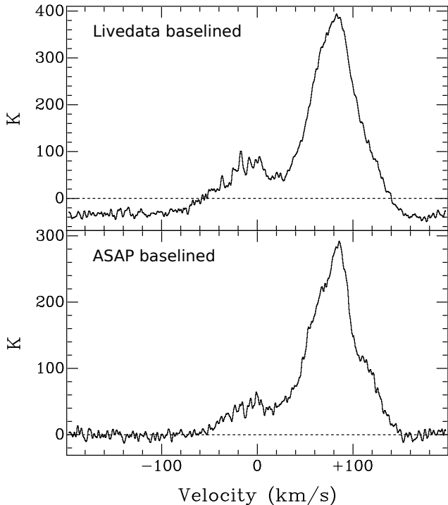
Figure A1. Integrated spectrum measured from an area of emission close to the Galactic centre. The spectrum in the top panel is drawn from the data baselined using only a 1 st order polynomial in LIVEDATA. The spectrum in the bottom panel has had further baselines subtracted using the ASAP fitting software.
