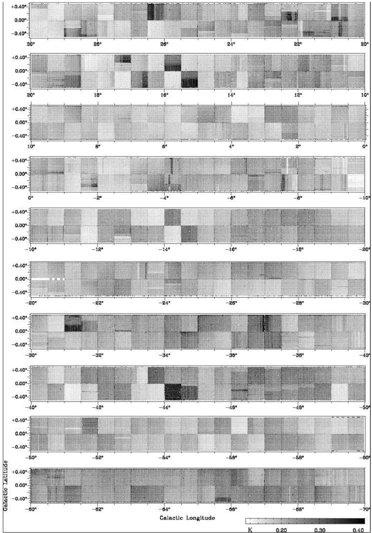
Figure 7. Image of the root-mean-squared noise temperature in T_{\text{mb}} units for the entire HOPS region made from the \text{NH}_3 (1,1) data. Individual observing blocks are visible as 0.5^\circ chequered squares, while scanning artifacts present as lines of high or low noise in Galactic l and b . The median root-mean-squared noise is 0.20 \text{ K} \pm 0.05 \text{ K} , where the uncertainty is the FWHM of the total noise distribution (also see Figure 8).
