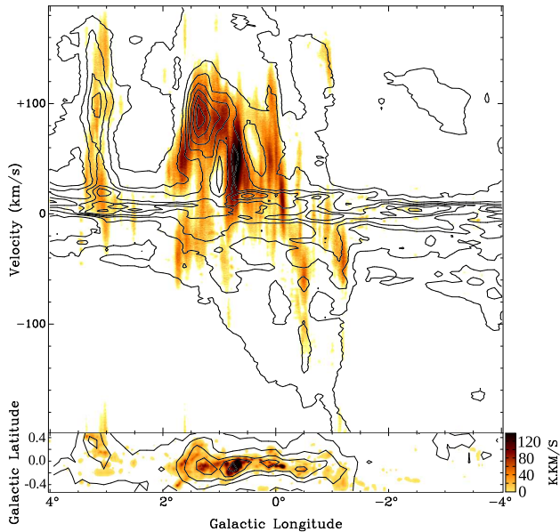
Figure 5. Detail of the longitude-velocity diagram showing the Galactic centre region (top). \text{NH}_3 (1,1) emission is shown in colour scale and the Dame et al. (2001) CO (1–0) contours are overplotted. While the overall emission morphology of both molecules is similar, the brightest peaks are offset in l and v . The emission seen at v < -170 \text{ km s}^{-1} is due to broad linewidth \text{NH}_3 (2,2) emission encroaching on the \text{NH}_3 (1,1) pass-band. The bottom panel shows the \text{NH}_3 (1,1) integrated intensity map for the same l range.
