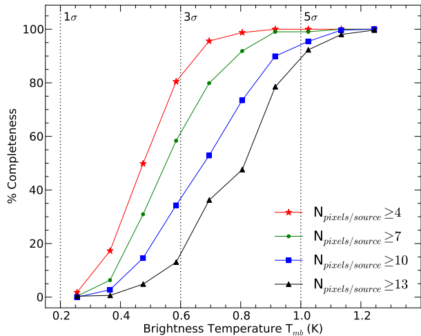
Figure 12. This figure shows the percentage completeness as a function of peak brightness temperature. The four curves illustrate the effect of varying the minimum number of spatial pixels required in a detection.
