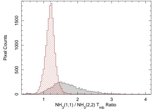
Figure 4. Plots of the brightness ratio T_{\text{mb},(1,1)}/T_{\text{mb},(2,2)} for every emitting voxel ( l - b - v data element) with T_{\text{mb}} > 3\sigma in both HOPS \text{NH}_3 datasets. The hatched histogram includes only voxels from the CMZ ( |l| < 2^\circ ) while the solid histogram includes the remaining emission from the outer Galaxy.
