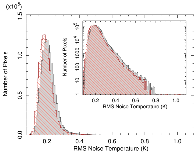
Figure 8. Histograms of the RMS noise temperature for all ( l, b ) spatial pixels in the \text{NH}_3 (1,1) and (2,2) data (grey-shaded and hatched histograms, respectively). The noise temperatures were determined from the line-free channels in the spectra. Inset is the same histogram, but with a logarithmic scaling on the Y-axis to enhance the view of the high-noise tail.
