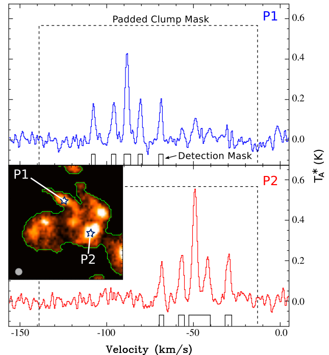
Figure B1. The inset image shows an integrated intensity map of \text{NH}_3 emission in the G333 cloud. The green contour represents the cloud boundary. DUCHAMP detects each of the \text{NH}_3 (1,1) spectral line components individually (top and bottom panels), however, the sub-clouds overlap both spatially and in velocity and are hence catalogued as a single merged cloud.
