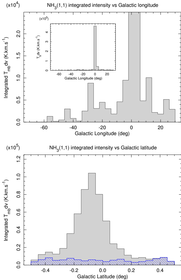
Figure 3. The top panel shows the sum of the \text{NH}_3 (1,1) integrated intensity over the survey region as a function of Galactic longitude in four-degree bins. The longitude bin covering the Central Molecular Zone (CMZ, -2^\circ < l < 2^\circ ) peaks at \int T_{\text{mb}} dv = 4.65 \times 10^5 \text{ K km s}^{-1} and the y-axis scale has been truncated so as to show the remainder of the emission. The inset shows how the plot appears scaled to the full \int T_{\text{mb}} dv range. In the bottom panel is a similar plot of \int T_{\text{mb}} dv versus Galactic latitude. The filled grey histogram includes all emission, while the hatched histogram includes only emission outside the CMZ.
