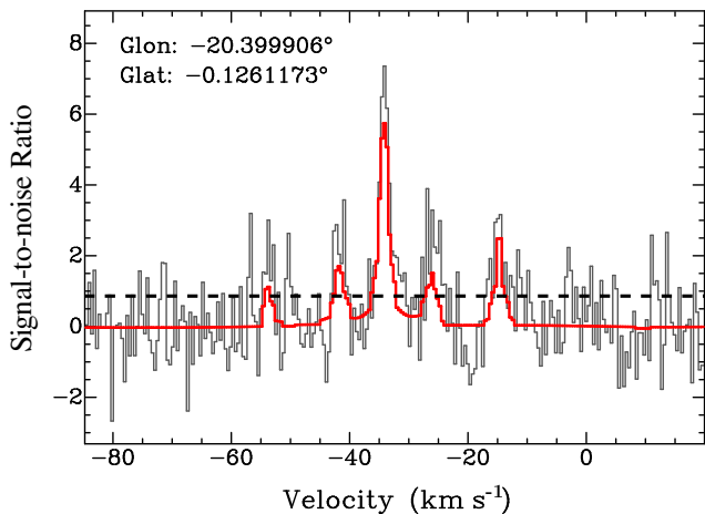
Figure 9. Example signal-to-noise spectrum (grey line) extracted from a single pixel with the wavelet-reconstructed spectrum overlaid (red-line). DUCHAMP does an excellent job of suppressing the noise allowing the use of a low threshold: 0.8\sigma in this case.
