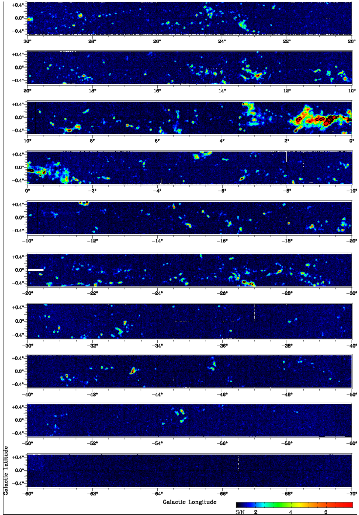
Figure 1. Map of the peak \text{NH}_3 (1,1) signal-to-noise (S/N) across the HOPS survey area. The map was made by smoothing the S/N cube spatially (final beam FWHM=2.5 arcmin) and in velocity (hanning-window=5) and measuring the peak brightness in each spectrum. An approximate brightness temperature scale may be found by multiplying by the average root-mean-squared noise temperature ( \sigma_{T_{\text{mb}}} = 0.20 K).
