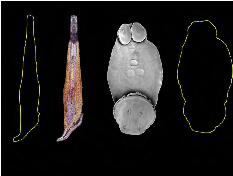
Figure 15. Images to show the distinctly different shapes of Zeuxapta seriolae (left) and Benedenia seriolae (right). In a revised version of BEAST, the shape descriptor ‘FCircle’ ( = [4 \times \pi \times \text{area}] / \text{perimeter}^2 ), which is an estimate of the sphericity of an object, was used in combination with other shape descriptors in a sub-routine to better separate mixed samples and provide separate summary statistics for each fluke species.
