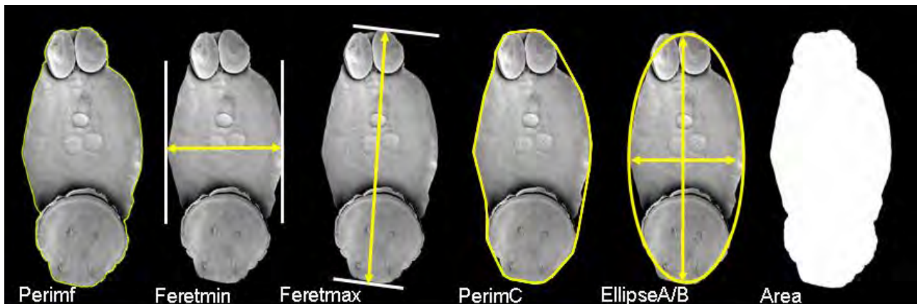
Figure 9. Examples of some of the shape descriptors used to characterise each individual of Benedenia seriolae (skin fluke) identified by the BEAST macro.
