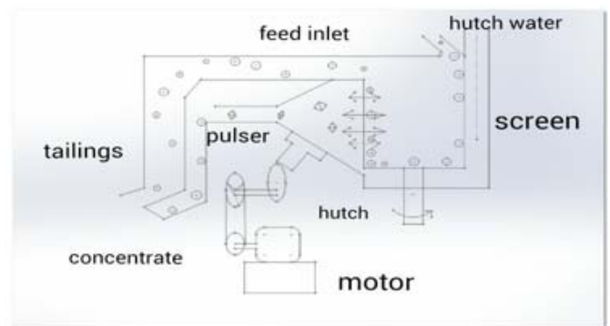
Figure 3: diaphragm pulsed with centrifugal effect separator
