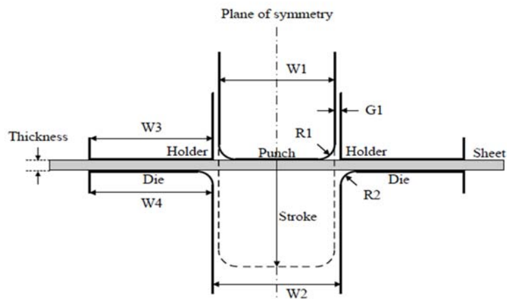
Figure 2. Schematic of a mechanical U – bending setup showing the punch, sheet and the die [1]
