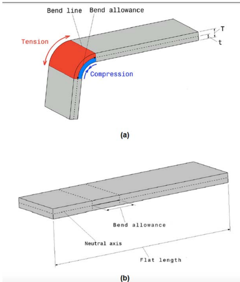
Figure 1. Schematic of the tension and compression during bending of the sheet [6]
