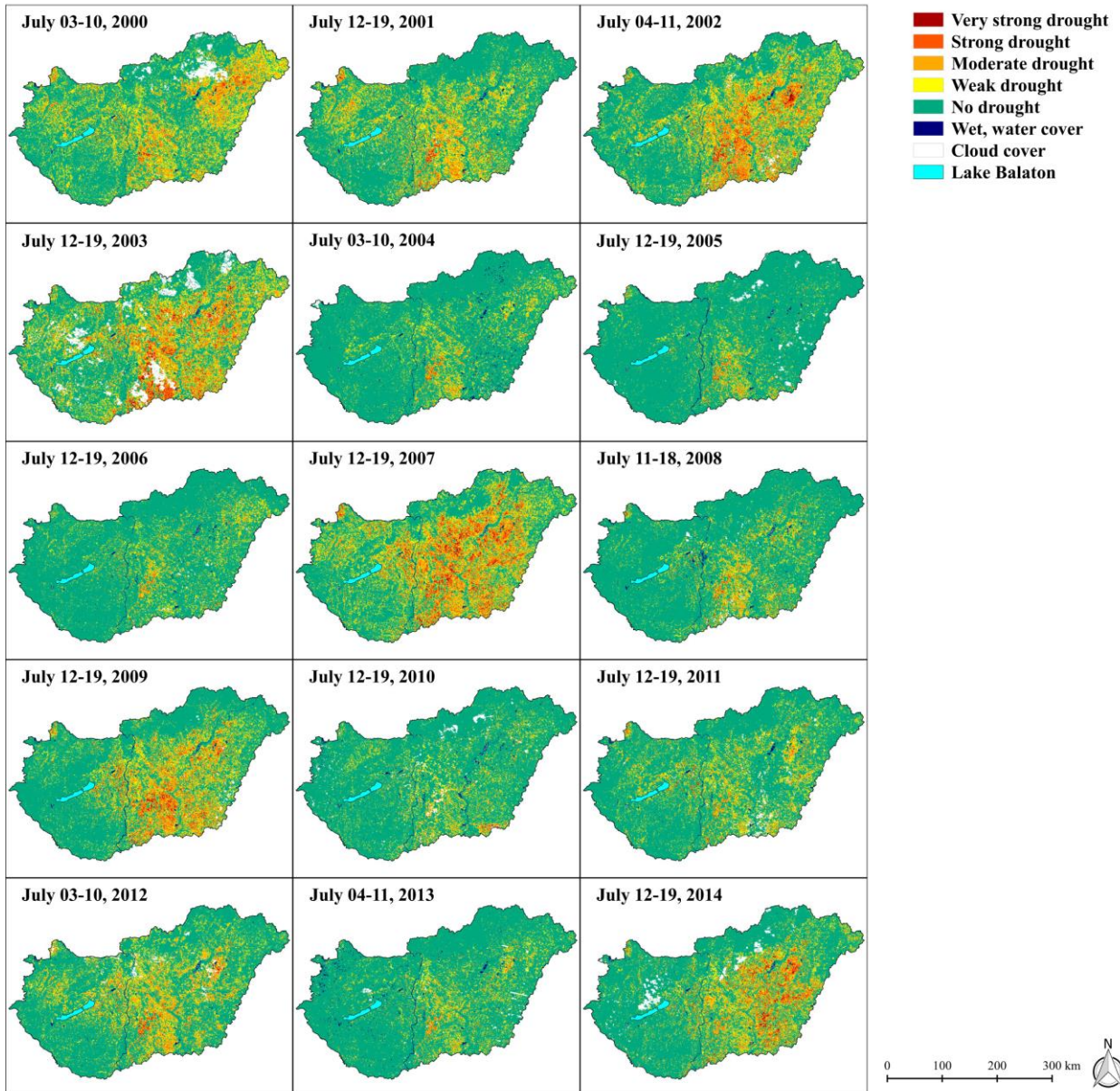
Fig. 4 Geographic distribution of drought areas according to DDI in July
