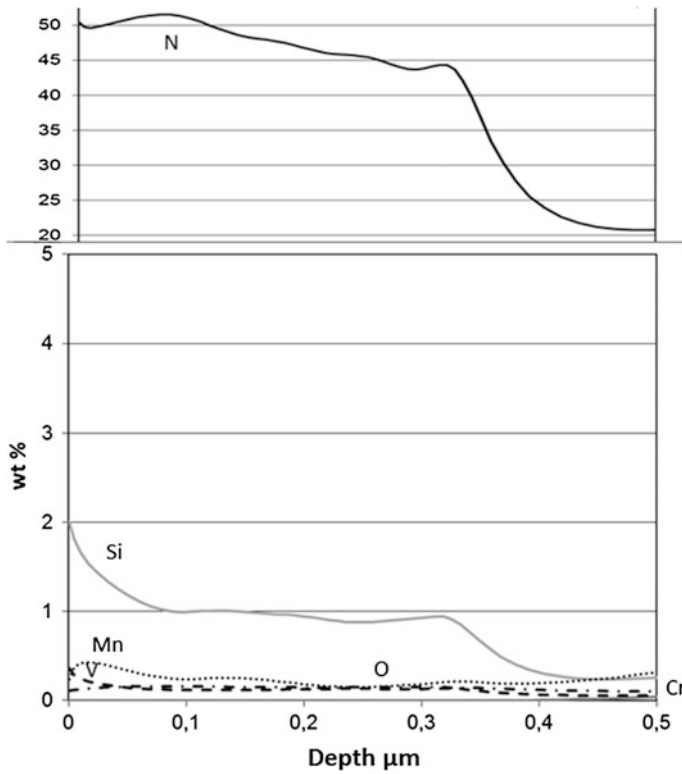
Fig. 3 GD-OES spectra of the 42CrMo4 alloy with oxide-free nitride coating
