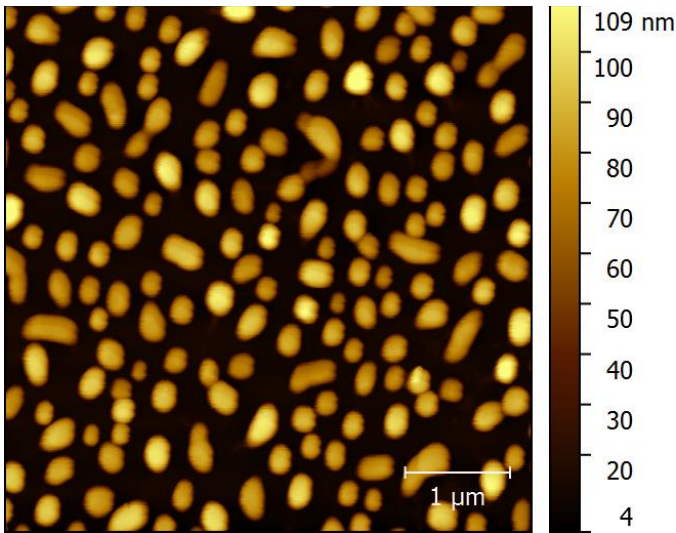
Fig. 4. Tapping-mode AFM topography image of gold nanoisland prepared by 120 min thermal annealing, measured with a blunt AFM tip. Image size: 5 \mu\text{m} x 5 \mu\text{m}
