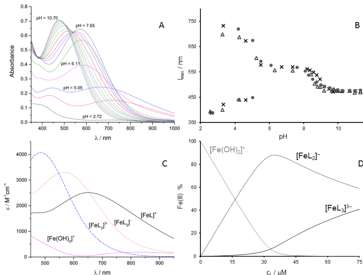
Figure 3. UV-Vis absorbance spectra recorded for the iron(III) – 6c (1:3) system at various pH values (A) and the \lambda_{\max} values at 1:3 (●), 1:2 (x) and 1:1 (Δ) metal-to-ligand ratios (B) ( c_L = 1.06 \text{ mM} ). Calculated molar absorptance spectra of the individual complexes of 6c (C). Concentration distribution curves for the iron(III) – 6c system at various total concentrations of the ligand at a constant concentration of iron(III) and at pH 8.0 (D). ( c_L = 0 - 75 \text{ } \mu\text{M} ; c_{\text{Fe(III)}} = 15 \text{ } \mu\text{M} ; \text{pH} = 8.0 ; I = 0.10 \text{ M (KCl)} ; T = 25 \text{ } ^\circ\text{C} )
