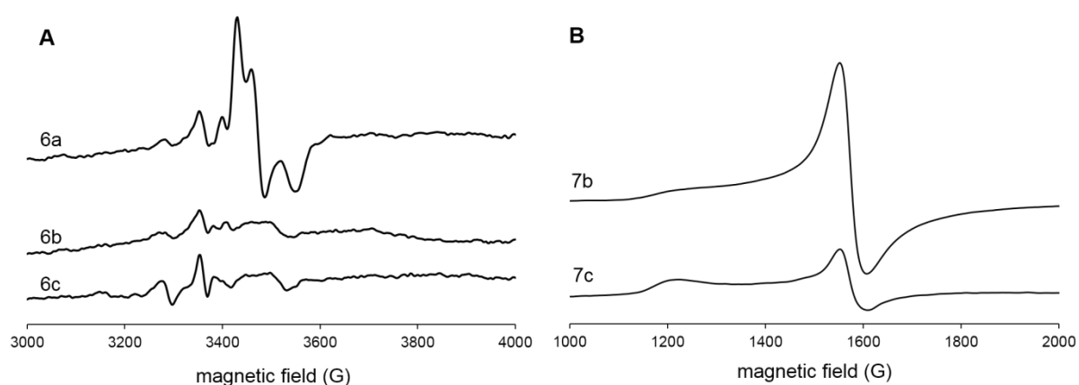
Figure 2. ESR spectra of the ligands, 6a–c (A), as well as of the iron complexes, 7b and 7c (B), measured at 9.43 GHz and 90 \pm 1 K.
