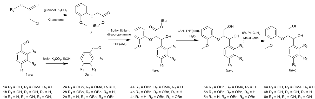
Scheme 1. Synthesis of \beta -O-4 type lignol compounds.
