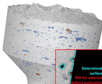
Figure 9. Detection of pores/defects on the external surface (in orange); internal pores are blue (Part V20).
