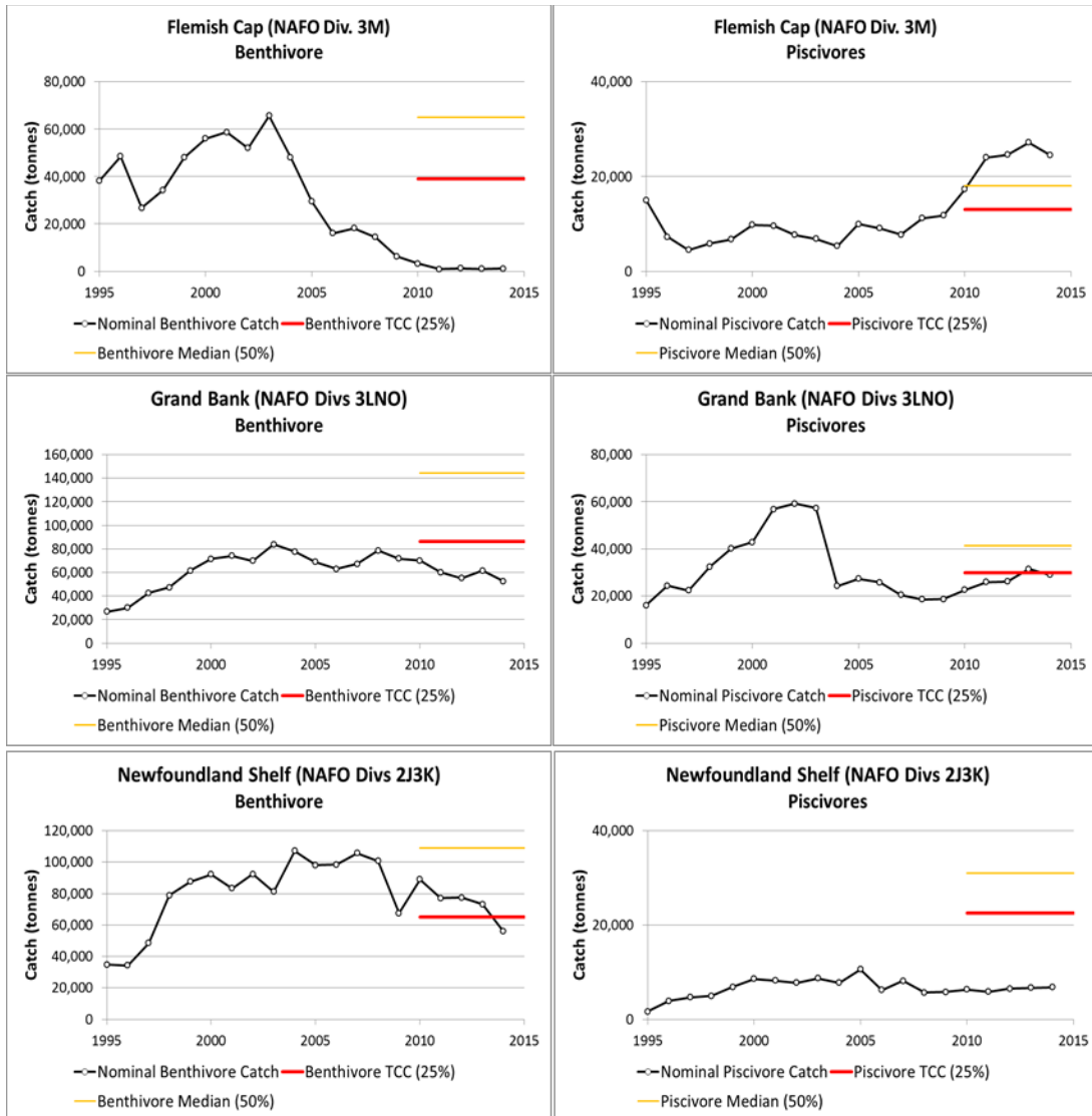
Fig.3. Time series of catches from the Flemish Cap (NAFO Div. 3M), Grand Bank (NAFO Div. 3LNO) and Newfoundland Shelf (NAFO Div. 2J3K) for benthivores and piscivores. The total catch ceilings (25th percentiles of the projections) and the median projected catch for each component are presented in each panel.
