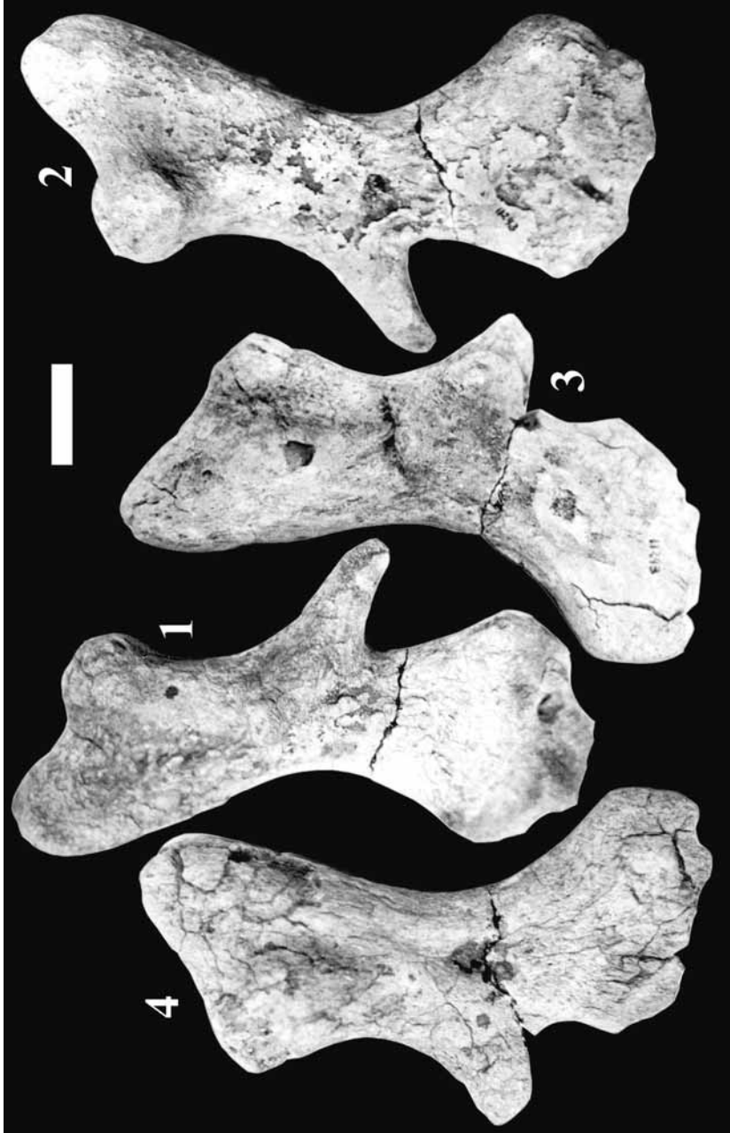
Plate 1. Original material of Psephophorus eocaenus in the Stuttgart Museum N.º 11243 a-b described by DACQUÉ, 1912. Figure 1 = humerus a dorsal, figure 2 = ventral, figure 3 = humerus b dorsal, figure 4 = ventral. Photographs by H.-V. Karl. Scale bar 1 cm.
