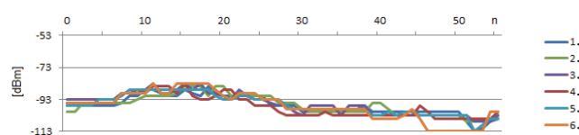
Fig. 2 Progress of the GSM signal availability on the selected route (author)
