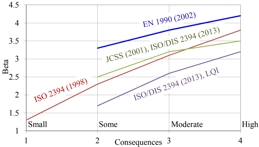
Fig. 3: Variation of \beta_{s0,1} for the ultimate limit states with a degree of failure consequences
