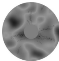
Fig. 6: Realization of a random field of local tensile strength f_t and cracks developed in the post peak stage of \sigma_1
