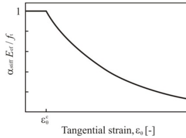
Fig. 2: Plot of the dependence of the residual stiffness \alpha_{\text{stiff}} on the tangential strain \varepsilon_0 , see Eq. (4)
