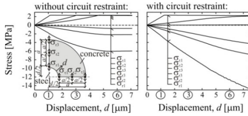
Fig. 4: Deterministic solution of the numerical models; comparison of restrained and non-restrained boundary conditions at the outer concrete boundary
