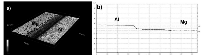
Fig. 3. a) Interface of explosive welded Mg/Al observed at magnification of 20× by 3D Optical Profiler SENSOFAR PLu neox. Average thickness of the bond is 45 μm b) height difference between Mg- (lower) and Al- (higher) plane is approximately 8 μm
