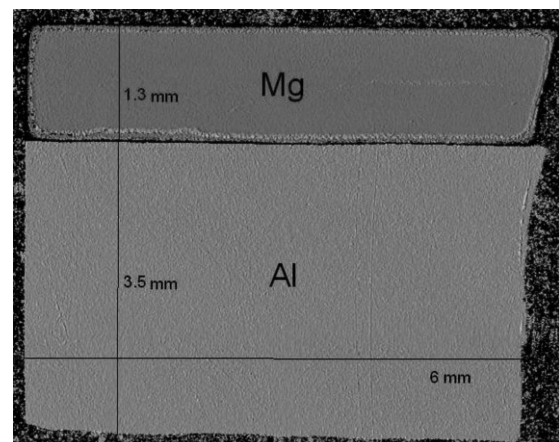
Fig. 1. Image of Mg/Al explosive welded bimetal from 3D Optical Profiler
