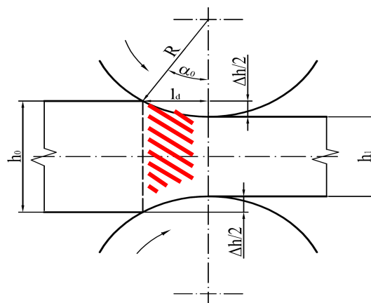
Fig.7. Deformation zone at longitudinal rolling.
