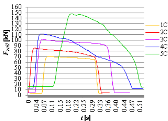
Fig.5. Graphical presentation of evolution of rolling force in time at the rolling speed of 0.7 \text{ m}\cdot\text{s}^{-1} [6].
