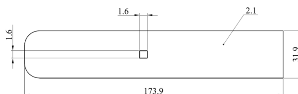
Fig.6. Diagram of the sample 1C with reduction of 0.38 mm with marked measured area of 1.6 \times 1.6 \text{ mm} .
