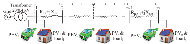
Fig. 2: A distribution feeder with PV and PEV systems and communication network.
