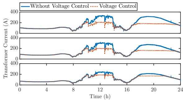
Fig. 13: Transformer current.
