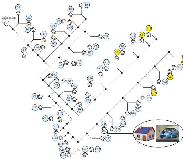
Fig. 4: The IEEE European LV test feeder.
