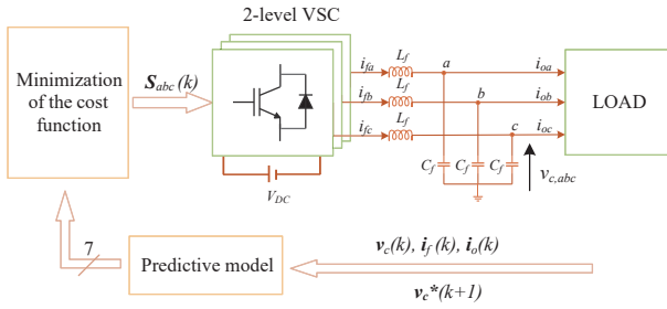
Fig. 1. Simplified scheme of model predictive control for 2-level VSC
