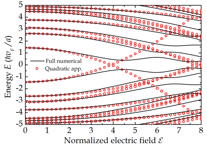
FIG. 3. Comparison of the approximate quadratic field dependence with the full numerical result.
