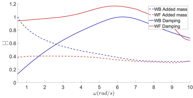
Fig. 13. Non-dimensional hydrodynamic coefficients for single WEC in wave flume and wave basin
