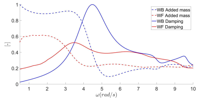
Fig. 16. Walls effect on hydrodynamic coefficients
