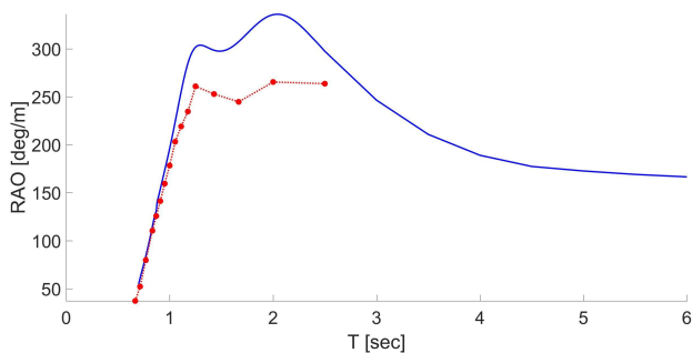
Fig. 23. Response Amplitude Operator of single WEC and surrounding structure in wave flume. Solid line corresponds to numerical model and markers to experimental data.
