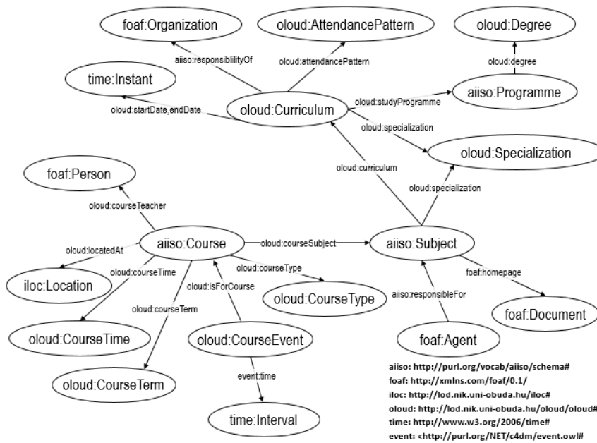
Fig. 2. Main classes and properties in OLOUD
