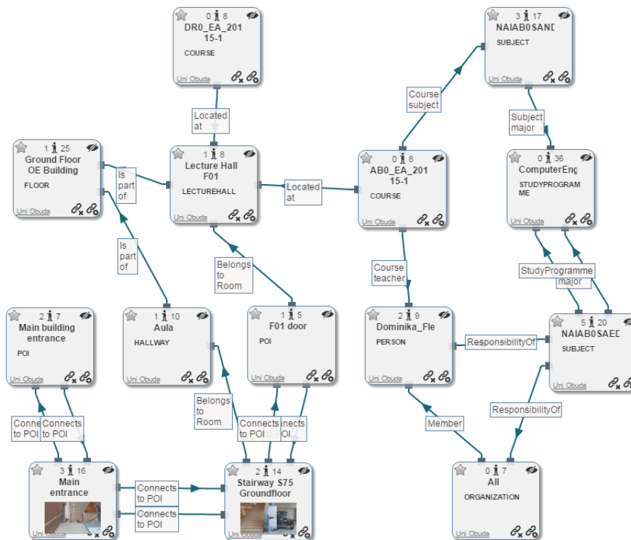
Fig. 3. Extract of the dataset presented with the Lodmilla browser
