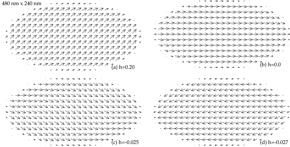
Figure 5. Magnetic configurations for a 480 \text{ nm} \times 240 \text{ nm} \times 24 \text{ nm} particle with magnetic field applied at +45^\circ above a horizontal axis pointing to the right. The arrows are the coarse-grained averages of 9 \times 9 groups of cells. In (a), the external field is h = 0.20 ; in (b) h = 0.0 ; (c) h = -0.025 , just before reversal; (d) h = -0.027 , just after reversal. Note the enhanced curvature of the field compared to that in the smaller particle in Figure 4.
