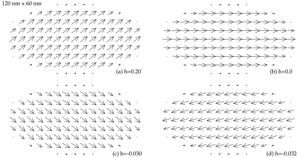
Figure 4. Magnetic configurations for a 120 \text{ nm} \times 60 \text{ nm} \times 6 \text{ nm} particle with magnetic field applied at +45^\circ above a horizontal axis pointing to the right. The arrows are the coarse-grained averages of 3 \times 3 groups of cells. In (a), the external field is h = 0.20 ; in (b) h = 0.0 ; (c) h = -0.030 , just before reversal; (d) h = -0.032 , just after reversal.
