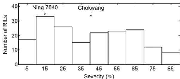
Figure 1 Frequency distribution of average leaf rust severity for the RIL population from Ning 7840/Chokwang in 2008 and 2009 experiments.
