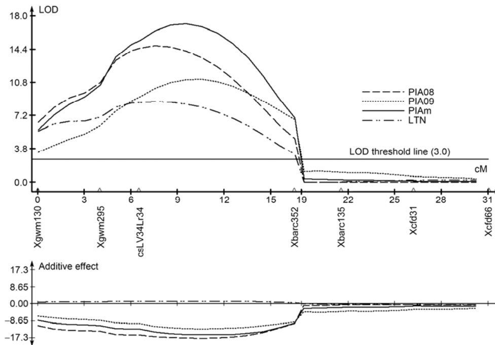
Figure 2 LOD curves for the Lr34 locus showing the QTL effect and location on chromosome 7D using percentages of infected flag leaf area (PIA) from 2008 (PIA08), 2009 (PIA09), the means over the two experiments (PIAm), and LTN data from 2009.
