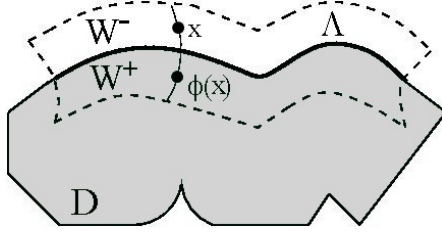
Figure 3: The sets W^+ , W^- , \Lambda and the bilipschitz map \phi .
