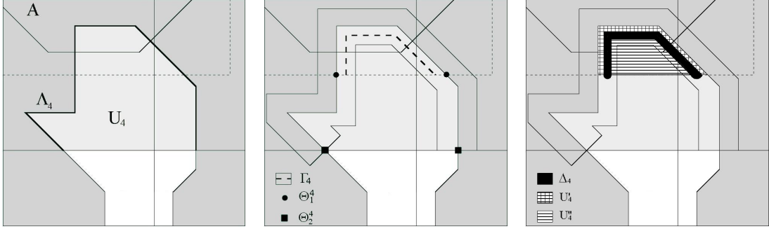
Figure 8: In this figure we present a step-by-step construction of the set \Delta_4 .
