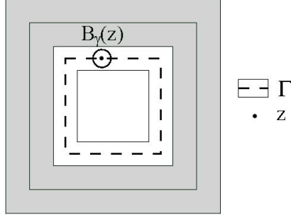
Figure 4: A point z \in \Gamma and the ball B_\gamma(z) . Here A, D and W are those shown in Figure 2.
