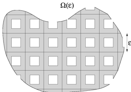
Figure 1: The perforated set \Omega(\varepsilon) , in the case n = 2 .
