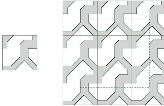
Figure 9: A periodic connected set with its periodicity cell. Notice that E \cap Q is not connected and that, in this case, \mathbf{k} = 2 .
