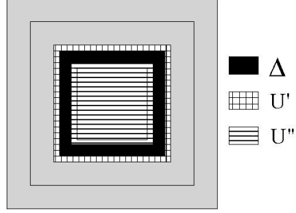
Figure 6: The sets \Delta , U' and U'' .
