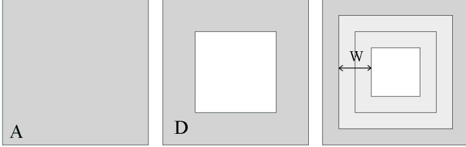
Figure 2: The set A ; the set D ; the neighbourhood W .
