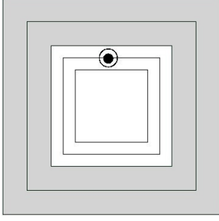
Figure 5: The ball B_{\frac{\gamma}{2}}(z) .
