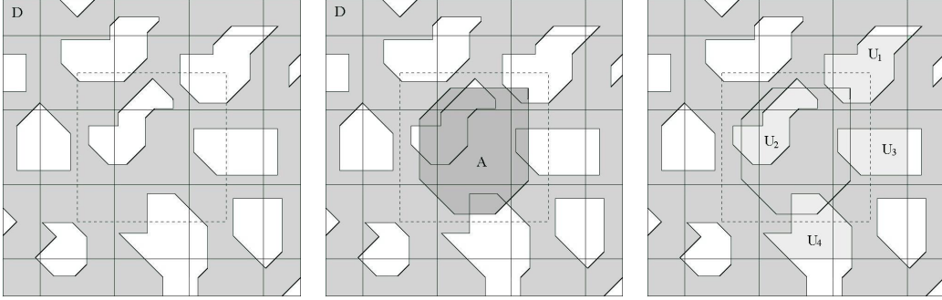
Figure 7: The set D ; the set A (here \mathbf{k} = 2 ); the sets U_i 's (notice that M = 4 ).
