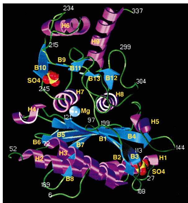
Figure 1 A ribbon diagram for the rabbit liver Fru-1,6-Pase monomer. Secondary structure elements defined in Table 4 are shown in magenta ( \alpha -helix), blue ( \beta -strand) and green (loops). This figure was drawn using SETOR (Evans, 1993).
