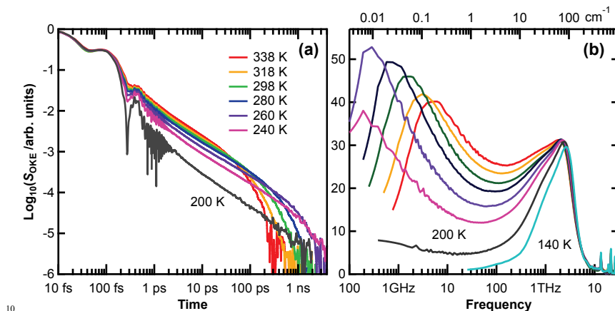
Fig. 3 (a) Time-domain OKE signal for propylammonium nitrate for seven temperatures between 200 K and 338 K. The fast and slow dynamics signals are joined at 5 between 5 and 7 ps. (b) The imaginary part of the spectrum yielded by a Fourier transform deconvolution of (a).
