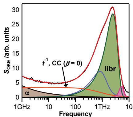
Fig. 4 Fit (red) of the OKE spectrum (black) for PAN at 200 K. CC is the Cole-Cole function with \beta = 0 described in the text.
