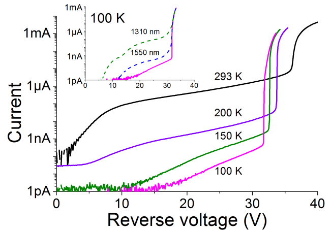
Fig. 3. Dark reverse current versus voltage characteristics at temperatures between 100 K and room temperature of a 25\text{-}\mu\text{m} -diameter SPAD. The inset demonstrates the dark current at 100 K (solid magenta line) and also the photocurrent at wavelengths of 1310 nm (dashed green line) and 1550 nm (dashed blue line).
