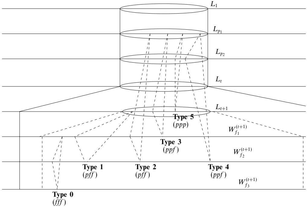
Figure 9.1. Different types of triple systems considered
