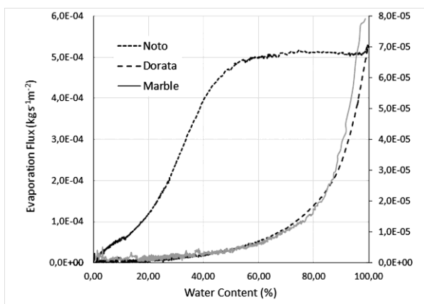
Fig. 4 Evaporation fluxes of three stones under controlled environmental conditions ( T=25^{\circ}\text{C} ; \text{RH}=50\% ) versus relative water content. The graphic has different scales of Noto stone (on the left) and of Dorata and marble (right)
