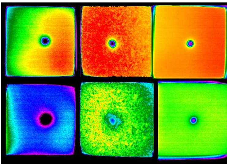
Fig. 6 Thermal images shot at the initial moment of spilling the drop on the stone surface (top line) and 10 minutes after or when the drop geometry became stable (bottom line). From left to right: Noto calcarenite, Dorata Sandstone and marble. Range of temperature 25.0-32.0°C; emissivity ranging between 0.89 (Dorata and Noto) and 0.95 (Prilep Marble).
