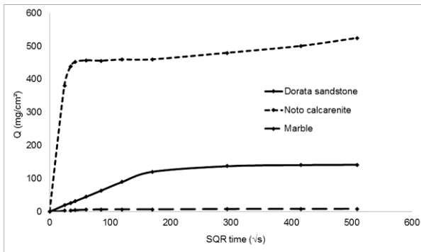
Fig. 3 Water absorption by capillarity (Q) of Dorata sandstone, Noto calcarenite, Prilep marble.
