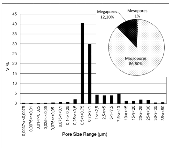
Fig. 1 Noto calcarenite, percentage of total volume (V%) as function of ranges of pores radius.
