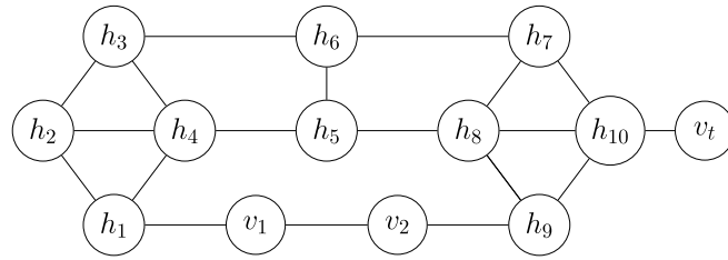
Fig. A.17. Example of construction used in the proof of Theorem 11 : the Hamiltonian path \langle h_1, h_2, h_3, h_4, h_5, h_6, h_7, h_8, h_9, h_{10} \rangle on G_H is given, as well as covering route r_1 with r_1(0) = v_1 and T(r_1) = T . It can be observed that there is another Hamiltonian path for G_H , i.e., \langle h_9, h_8, h_5, h_4, h_1, h_2, h_3, h_6, h_7, h_{10} \rangle , allowing covering route r_2 with r_2(0) = v_2 and T(r_2) = T . Notice that, if we remove the edge (h_5, h_8) , then covering route r_2 such that r_2(0) = v_2 and T(r_2) = T does not exist.
