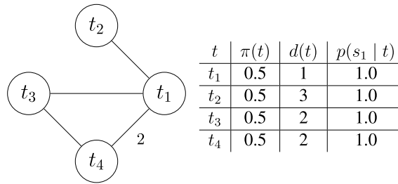
(a) Equation 1 holds for \alpha \leq 0.25 .
