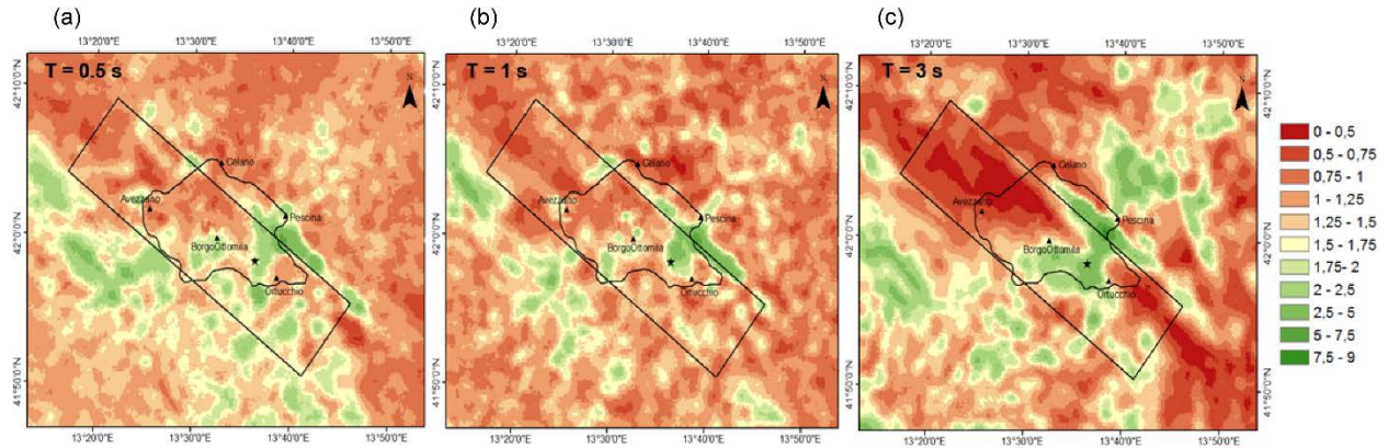
Fig. 9. Spatial distribution of the ratio between FN and FP component of 5% damped response acceleration spectrum for T = 0.5 s (a), 1 s (b), 3 s (c).
