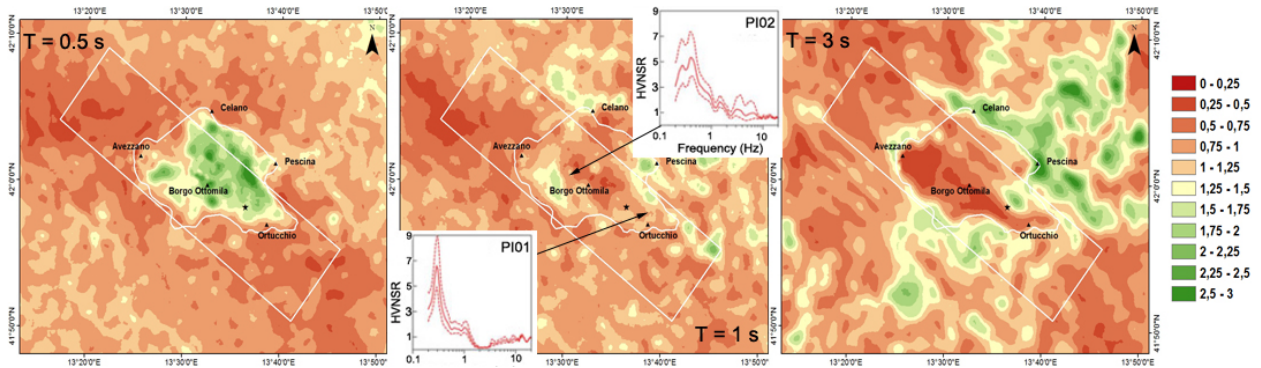
Fig. 12. Spatial distribution of the ratio between Z and the geometric mean of FN and FP components of 5% damped response acceleration spectrum for T = 0.5 s (a), 1 s (b), 3 s (c). In the (b) panel, the horizontal-to-vertical spectral ratios at two locations of the array investigated by [11] are shown.
