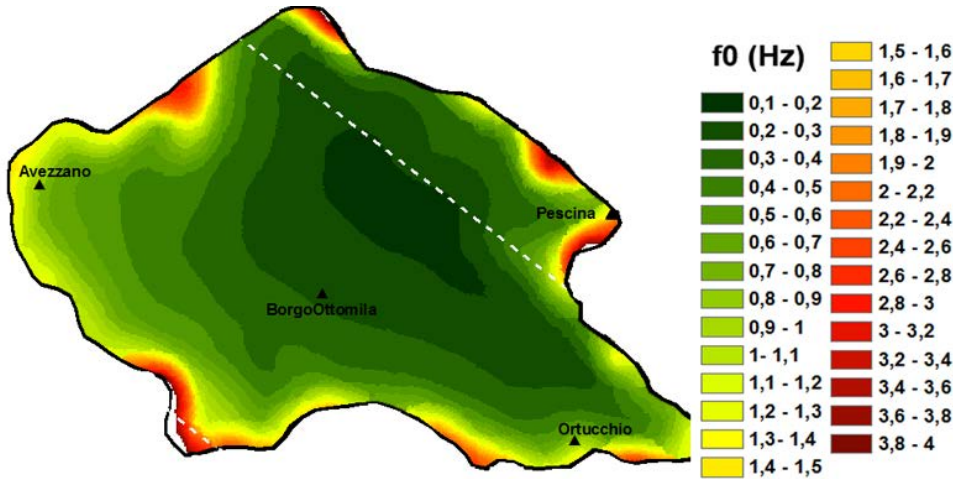
Fig. 15. Map of 1D natural frequency of vibration f_0 of the Fucino basin.
