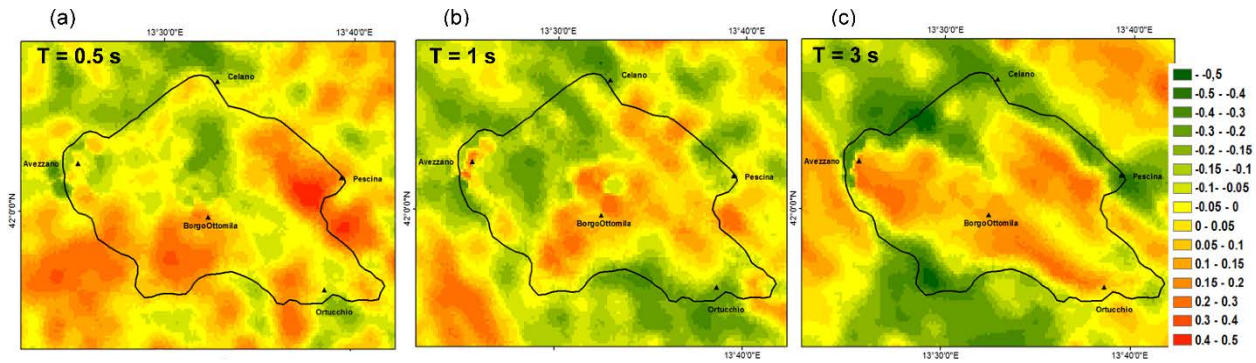
Fig. 16. Map of residuals \varepsilon = \log_{10}(S_{a_{sim}}(R,T)/S_{a_{avg}}(R,T)) , where S_{a_{avg}}(R,T) is the average simulated spectral ordinate at period T and at distance R=R_{LINE} , either within the basin or on rock, and S_{a_{sim}}(R,T) is the corresponding value simulated at the specific location. Three values of period are considered: T = 0.5 s (a), 1 s (b), 3 s (c).
