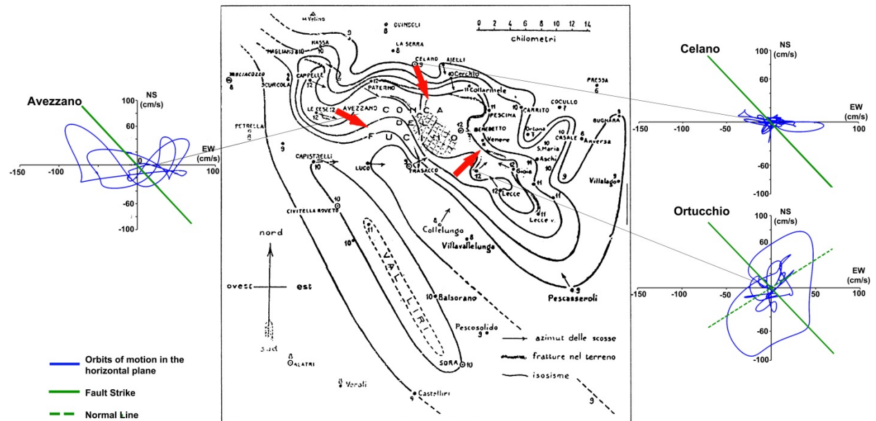
Fig. 10. In the background (Fig. center), the isoseismal map compiled by [4] after the earthquake, together with the arrows denoting the prevailing “azimuth of shaking”. Superimposed are the plots of the orbits of ground motion in the horizontal plane, computed by the numerical simulations, at the sites of Avezzano, Ortucchio and Celano.
