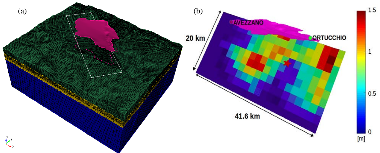
Fig. 5. (a) 3D computational mesh adopted for the numerical model along with the projection of the seismic fault responsible of the January 13 1915 earthquake and buried topography, corresponding to Quaternary sediments in Fig. 2. (b) Assumed slip distribution to model the earthquake fault rupture, as described in Section 3.
