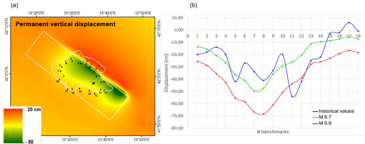
Fig. 6. (a) Map of permanent vertical displacements computed by SPEED for a simulated earthquake magnitude M_W 6.7, with the slip distribution in Fig. 5. (b) Comparison of the historical values from geodetic measurements [31] (blue line), with the simulated permanent displacements obtained with M_W 6.7 (green line) and M_W 6.9 (red line).
