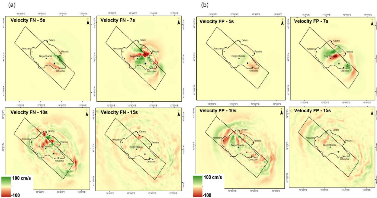
Fig. 7. Snapshots of the computed velocity field at different time instants T = 5, 7, 10, 15 s. (a) Fault Normal (FN) component. (b) Fault Parallel (FP) component.
