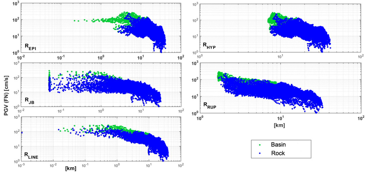
Fig. 14. Variability of PGV (FN component) with respect to different distance metrics. Values are expressed in cm/s.
