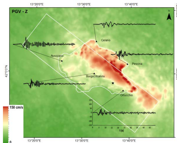
Fig. 11. PGV map for the Z component, in the same format as Fig. 8.
