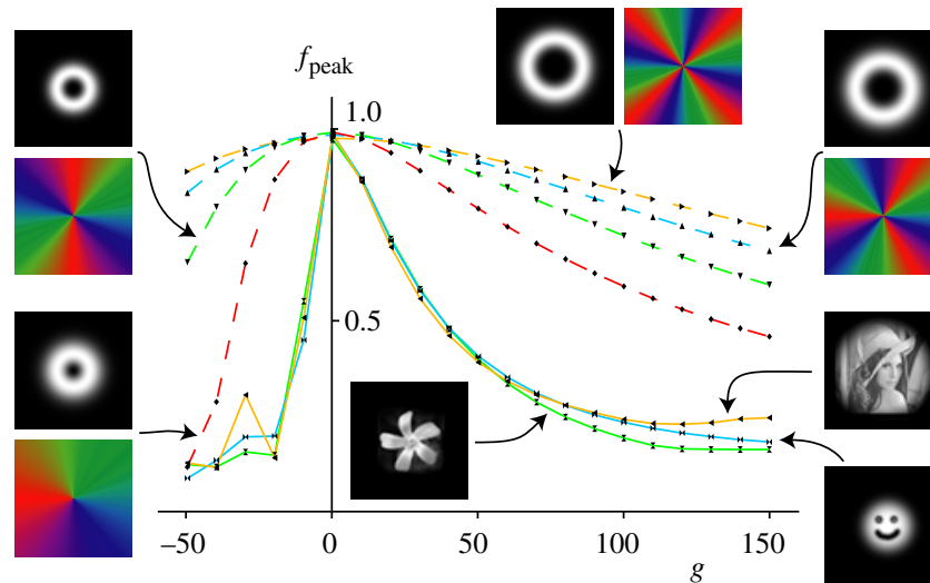
Figure 6. Maximum fraction in the state P of a BEC's wavefunction during simulated time evolution through T/2 , starting with the Fourier transform of P , as a function of g , for various choices of P . The insets show a greyscale representation of the central 20 \times 20 dimensionless units of the density of the state P for each curve, and a colour representation of the phase (unless the phase is uniform).
