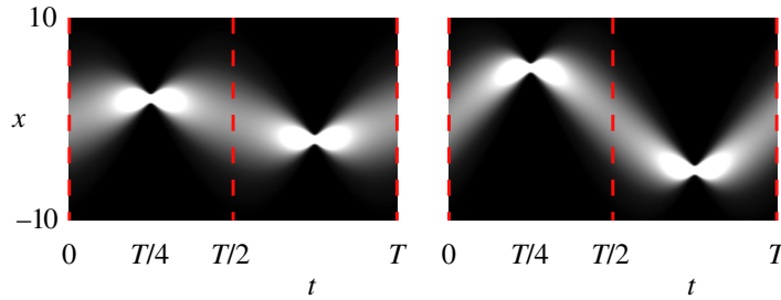
Figure 1. Dynamics of one-dimensional (1D) breathing dipole modes—approximations to a BEC’s Fourier components. The graphs show a greyscale representation of the density distribution along the x axis as a function of time, t , calculated using equation (3). At t = 0 , the wavefunction is a Gaussian of width 4 (in units of the dipole-mode width) with a transverse wavenumber k_x = 3 (left panel) and k_x = 5 (right panel). The time evolution of the probability density is plotted over one trap period, T . At t = T/4 , the width of the BEC has shrunk to one quarter of the dipole-mode width (generally it is inversely proportional to the width at t = 0 ) and its position is proportional to the transverse wavenumber at t = 0 , k_x . Every further quarter of a trap period corresponds to an additional Fourier transform.
