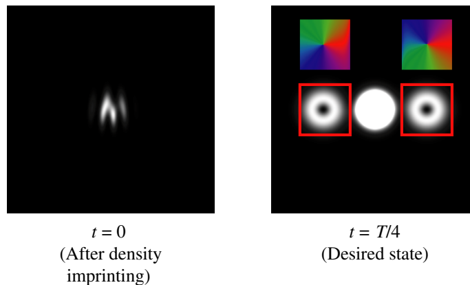
Figure 3. Shaping of a BEC in the Fourier domain. In this example, the phase and density of part of a pancake BEC was shaped into a vortex at t = T/4 after only the density of the BEC was manipulated a quarter of a trap period earlier ( t = 0 ). The state at t = 0 was calculated according to equation (6). At t = T/4 , about 85% of the remaining BEC is in the central peak, the rest is distributed equally between the doughnut-shaped vortices with circulation +1 and -1 on either side (about 7.5% each). A colour representation of the phase in the areas around both vortices, marked by red squares, is shown above the squares. The simulations for this figure were performed on a 256 \times 256 grid representing an area of 28 \times 28 dimensionless units.
