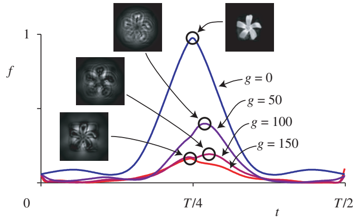
Figure 4. Time evolution of a BEC in a harmonic trap in terms of the Fourier transform of the initial wavefunction. The initial wavefunction ( t = 0 ) was set to the inverse Fourier transform of wavefunction P with a distinctive density distribution. The graph shows the fraction, f , of the wavefunction \psi(t) in the state P , calculated according to equation (7). The figure was calculated for various interaction strengths ( g = 0, 50, 100 and 150 ). In the interaction-free case ( g = 0 ), close to 100% of the BEC is in the Fourier transformed state, i.e. P , at T/4 . Insets show the density of the wavefunction corresponding to the peaks of the different curves, where for g = 0, 50, 100 and 150 respectively 97.5, 39.8, 19.3 and 16.3% of atoms are in the state P . The central squares of side length 20 dimensionless units are shown. Like those for figures 5 and 6, the simulations for this figure were performed on a 128 \times 128 grid representing a square of side length 40.1 dimensionless units.
