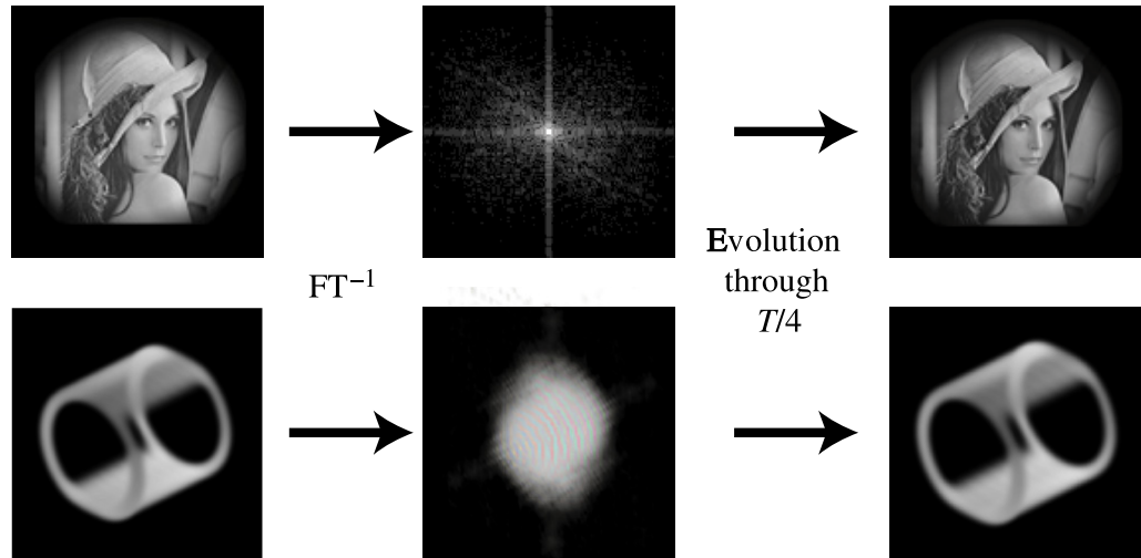
Figure 2. Simulated Fourier transform of non-interacting ( g = 0 ) trapped 2D (top panel) and 3D (bottom panel) BECs by waiting a quarter of the trap period, that is T/4 . In both cases, we set the initial wavefunction (centre; log plot over four orders of magnitude) to the (discrete) inverse Fourier transform of distinctive shapes (left panel)—a well-known photo in the 2D case and a shape that looks circular from one direction and square from another in the 3D case—and simulated their time evolution over T/4 , using a split-step technique. In the 2D case, the simulations were run on a grid of 96 \times 96 , representing a square of side length 34.7 dimensionless units. Density is represented as brightness (black represents zero density, white maximum density). In the 3D case, simulations were run on a 64 \times 64 \times 64 grid, representing a cube of side length 35 dimensionless units. Density is represented as white opacity in front of a black background; the graphs were created using the Volpack rendering software [8, 9].
