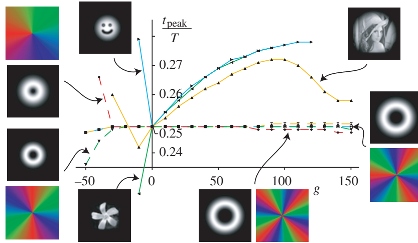
Figure 5. Time after which most of the BEC is in the Fourier transformed state for various wavefunctions (insets) as a function of the interaction strength g . Only the data points for which more than 20% of the BEC are in the Fourier transformed state are shown. Insets show a greyscale representation of the central 20 \times 20 dimensionless units of the density of the state P for each curve, and a colour representation (the colour range red \rightarrow green \rightarrow blue represents phases between 0 to 2\pi ) of the phase, unless the phase is uniform.
