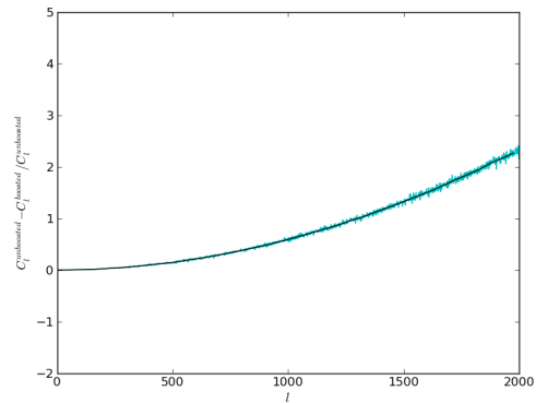
FIG. 3. Comparison of power spectra produced from a map that was not boosted versus a map that had been boosted and deboosted. The difference should be zero, as deboosting should return the map pixels to their original values. The difference shown is therefore due to pixelization effects. The blue line shows the difference for individual C_\ell s and the black line shows the difference in binned C_\ell s. Values are quoted in percent.
