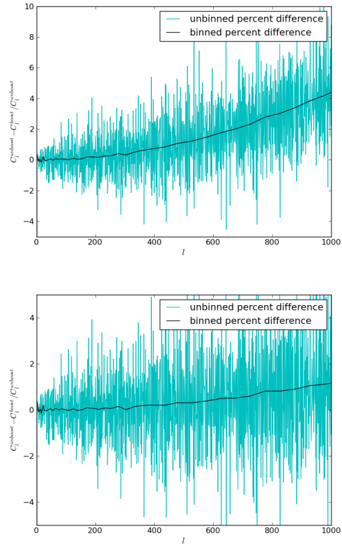
FIG. 6. Comparison of N_{\text{side}}=2048 (top) and N_{\text{side}}=4096 (bottom). These have been boosted and downgraded to N_{\text{side}}=1024 . Values are quoted in percent.
