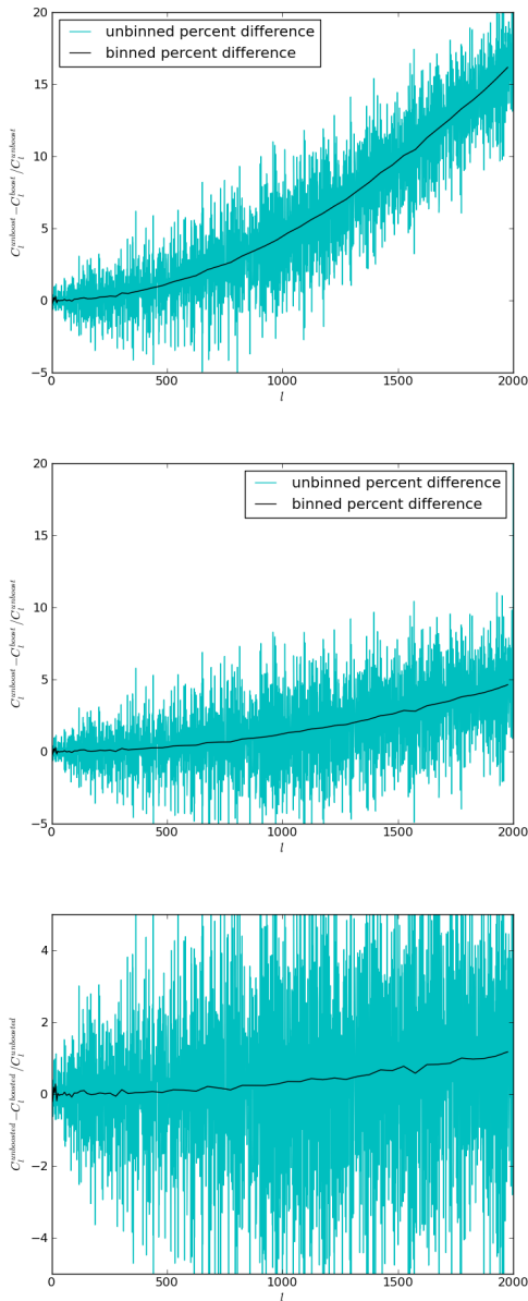
FIG. 2. Comparison of power spectra produced from boosted versus unboosted full-sky maps at N_{\text{side}}=2048 (top) 4096(middle) and 8192(bottom). The blue line shows the difference for individual C_\ell s and the black line shows the difference in binned C_\ell s. Values are quoted in percent.
