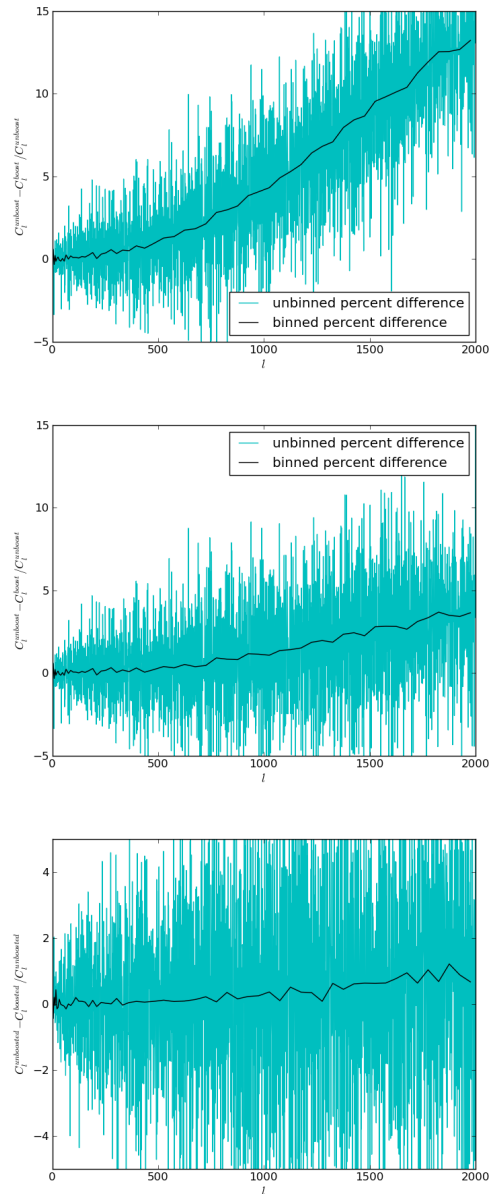
FIG. 8. Comparison of n_{\text{side}}=2048 (top), 4096(middle), and 8192(bottom). These have been boosted, downgraded to n_{\text{side}}=1024 , and masked with a galactic mask provided by LAMBDA. Values are quoted in percent.
