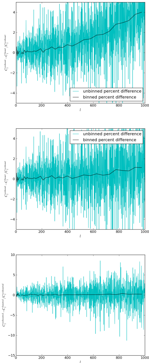
FIG. 7. Comparison of n_{\text{side}}=2048 (top), 4096(middle), and 8192(bottom). These have been boosted, downgraded to n_{\text{side}}=512 , and masked with a galactic mask provided by LAMBDA. Values are quoted in percent.
