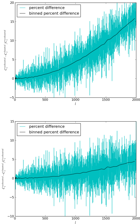
FIG. 9. Comparison of n_{\text{side}}=2048 (top) and n_{\text{side}}=4096 (bottom). These have been boosted and masked with a 20 degree isolatitude equatorial strip. Values are quoted in percent.
