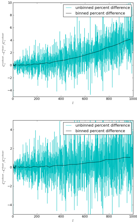
FIG. 5. Comparison of N_{\text{side}}=2048 (top) and N_{\text{side}}=4096 (bottom). These have been boosted and downgraded to N_{\text{side}}=512 . Values are quoted in percent.
