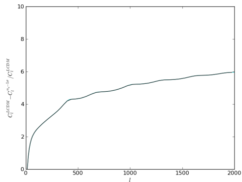
FIG. 4. Percent difference between a power spectrum generated by CAMB [11] with n_s - 1\sigma and a standard LCDM power spectrum. Values are quoted in percent.
