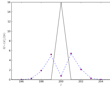
FIG. 1. Comparison of boosted (blue dashed line) and unboosted (black solid line) temperature power spectra from a simulated sky at N_{\text{side}}=512 with all power in the \ell = 200, m = 0 mode to the exact solution. Differences between the numerically boosted result and the exact solution (magenta dots) are predominantly due to map resolution effects. A \beta value of .01 was used to obtain these results.
