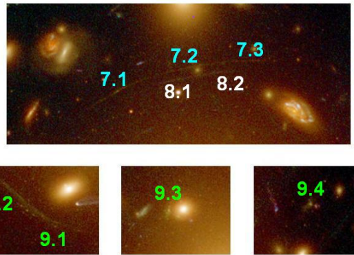
FIG. 10.— Stamp images of some of our newly identified multiple-images, seen more clearly in this color-composite image constructed from 16 HST bands ranging from the UV to the IR. As can be seen, systems 7 and 8 follow the same symmetry and are clearly multiple images as supported also by our mass model and photo- z 's (see Table 2). In system 9, images 9.1 and 9.2 are clearly multiply-lensed to form the greenish-looking arc, while 9.3 and 9.4 are the most likely counter images as predicted by our model and coherent photo- z 's seen in Figure 11. Other similar looking objects are seen close to these images which might be the actual counter images, but such a degeneracy does not affect the mass model in a noticeable way.
