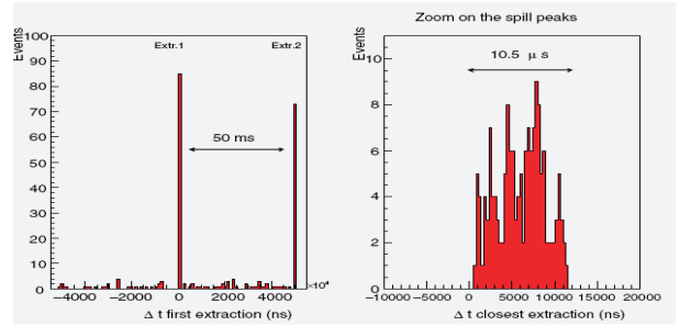
Figure 2: CNGS beam time structure seen in OPERA
