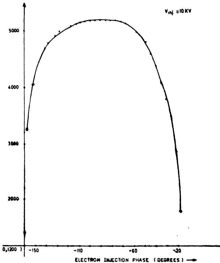
Figure 5. Energy spectrum.
