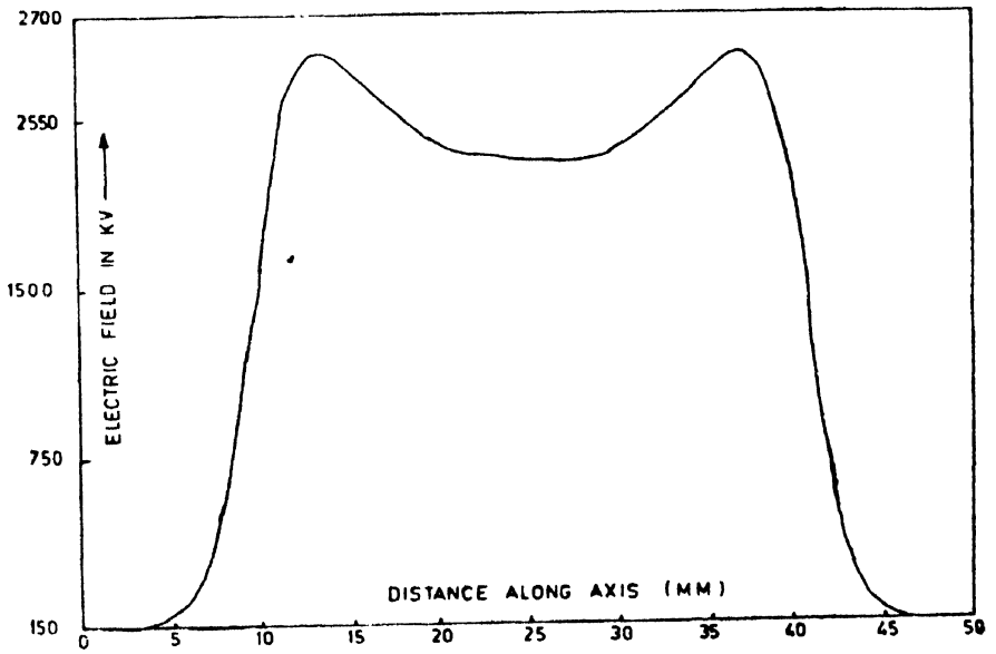
Figure 2. Electric field variation along linac axis.
