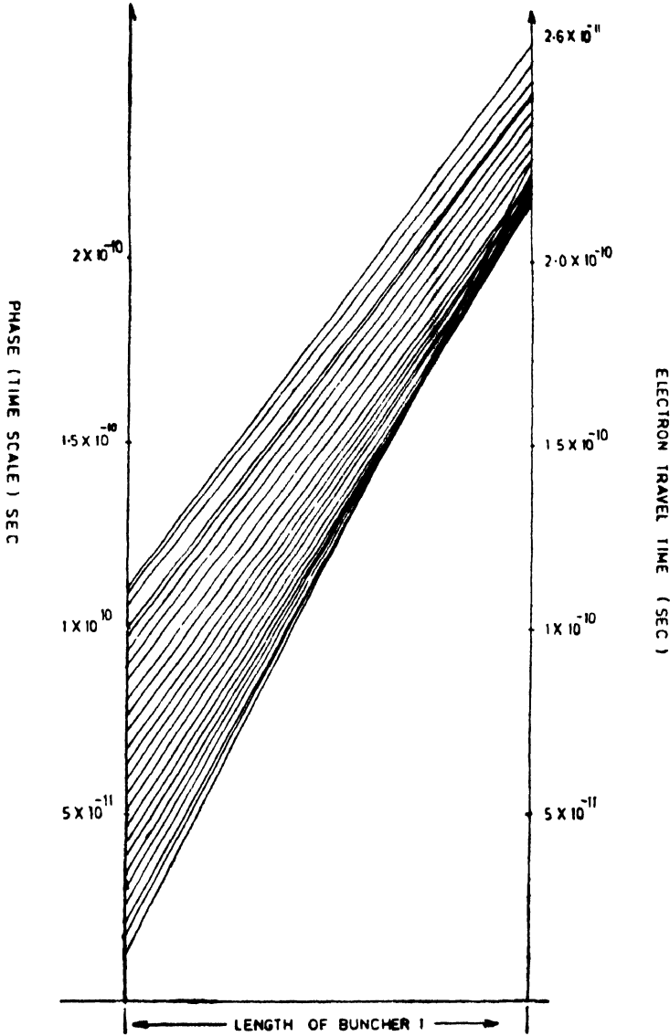
Figure 4. Electron bunching process.
