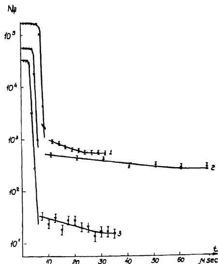
Figure 2. Time distribution of fission fragments in reactions
