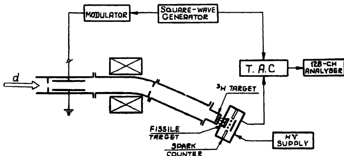
Figure 1. A schematic diagram of the experimental set up.
