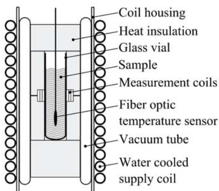
Figure S6. Conventionally built heating system
