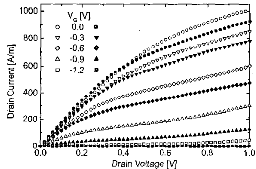
Figure 4 - I_d-V_d comparison for 120nm standard (transparent) and self-aligned devices (opaque)
