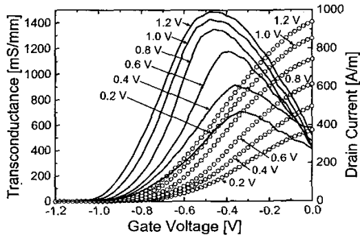
Figure 5 - I_d - V_g (circles) and transconductance (full lines) for a 120nm self-aligned device. Drain voltages indicated for each sweep.
