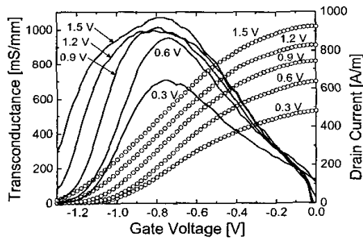
Figure 6 - I_d - V_g (circles) and transconductance (full lines) for a 120nm standard device. Drain voltages indicated for each sweep.
