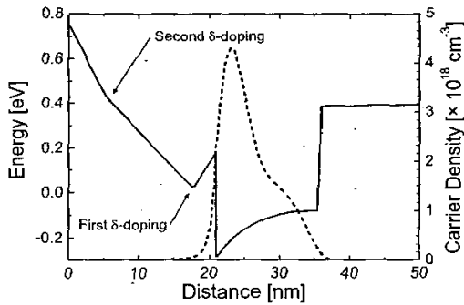
Figure 2 - Conduction band and carrier concentration profiles vs distance under the gate at V_g=0\text{V}
