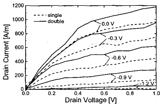
Figure 9 - Intrinsic I_d - V_d characteristics for a standard double-delta doped 120\text{nm} device compared with those for a single doped 120\text{nm} device. Both results were attained from calibrated MC device simulations.
