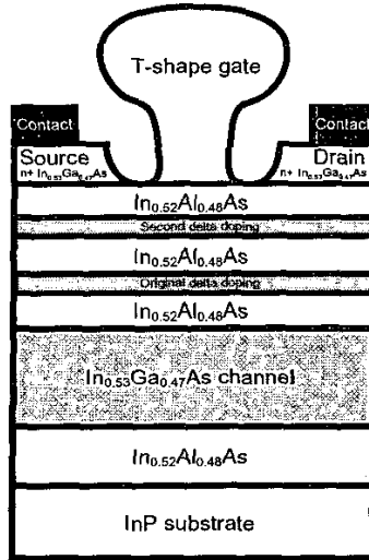
Figure 1 - Cross section of 120 nm gate device and layer structure with double-delta doping
