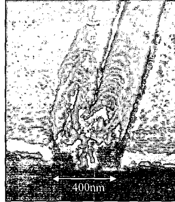
Figure 3 - SEM image of a self-aligned 120nm T-gate.
