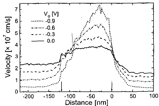
Figure 8 - Average velocity along the channel for a standard 120nm device at V_d = 1.0\text{V} . Gate voltages as indicated. The gate region is marked by arrows.
