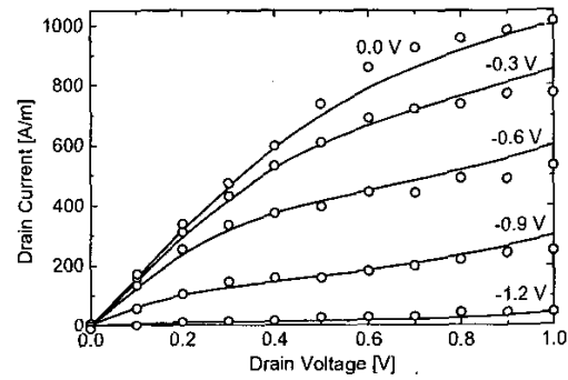
Figure 7 - Calibration of I_d - V_d characteristics obtained from MC device simulations (circles) against experimental data (full lines) for a standard 120nm device. Gate voltages are indicated for each sweep.
