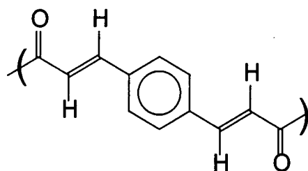
Figure 5.8 Main chain cinnamate polymers 10
