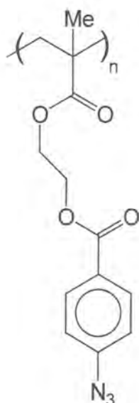
Figure 3.3 Poly(para-azidobenzoate-2-ethyl methacrylate)
