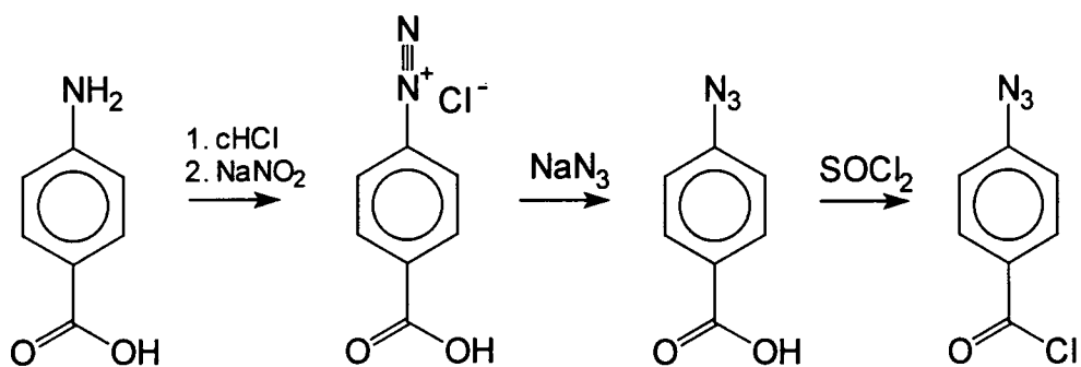
Figure 3.4 Formation of 4-Azidobenzoyl chloride
