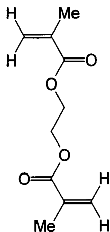
Figure 2.12 Ethylene glycol dimethacrylate
