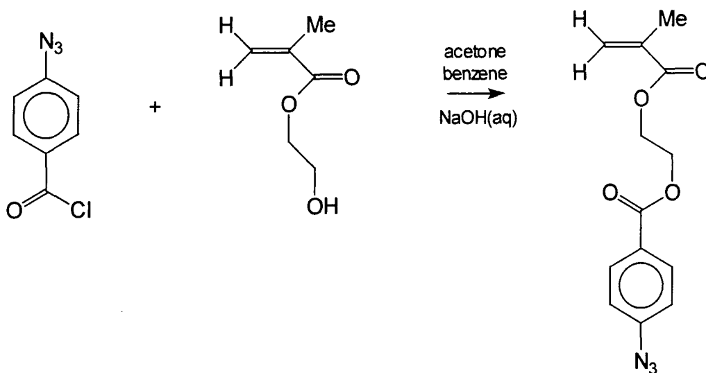
Figure 3.9 Monomer Synthesis 2
