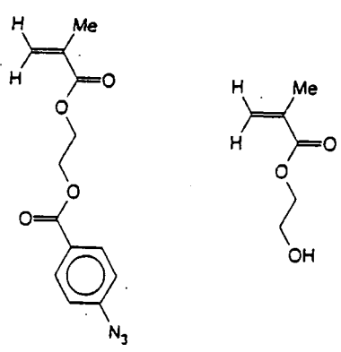
4. 4-Azidobenzoate-2-ethyl methacrylate + hydroxyethyl methacrylate
