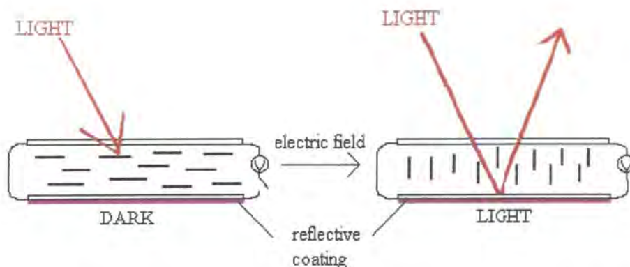
Figure 1.6 Switching of a Liquid Crystal Cell
