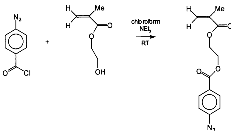
Figure 3.8 Monomer Synthesis 1
