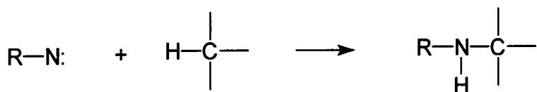
Figure 5.2 Insertion into C-H bonds
