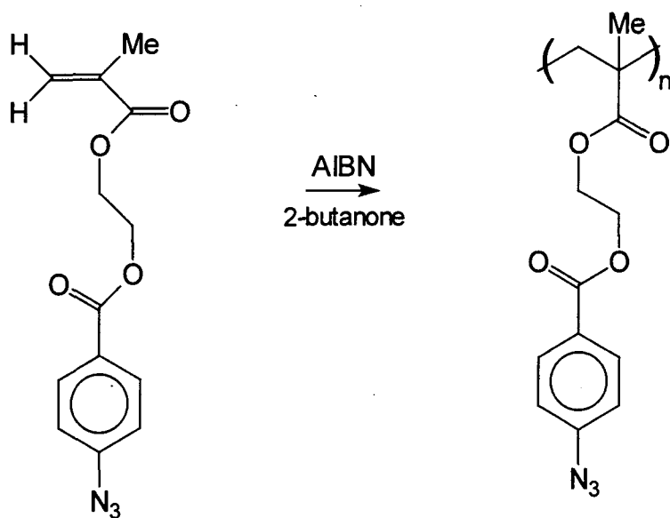
Figure 3.10 Polymerisation of the Azide Monomer
