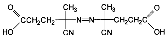
Figure 4.1 4,4'-Azobis-(4-cyanopentanoic acid)
