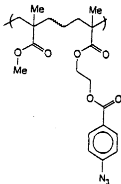
4. Poly(4-azidobenzoate-2-ethyl methacrylate-co-methyl methacrylate)
