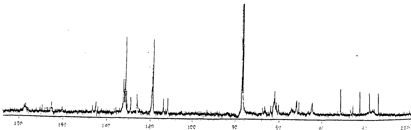
4. Poly(4-azidobenzoate-2-ethyl methacrylate-co-methyl methacrylate)
