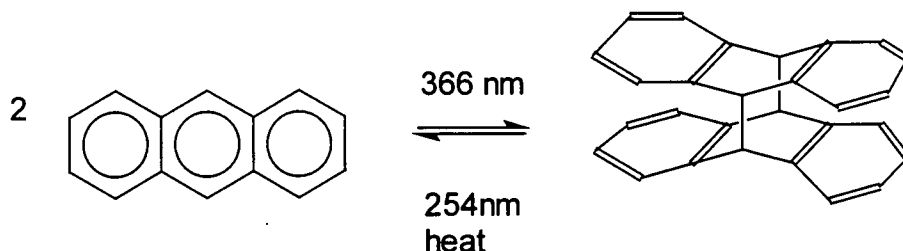
Figure 2.1 The dimerisation and cleavage of anthracene
