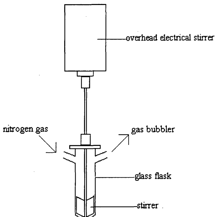
Figure 2.15 Bulk polymerisation apparatus
