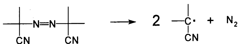
Figure 2.10 AIBN decomposition
