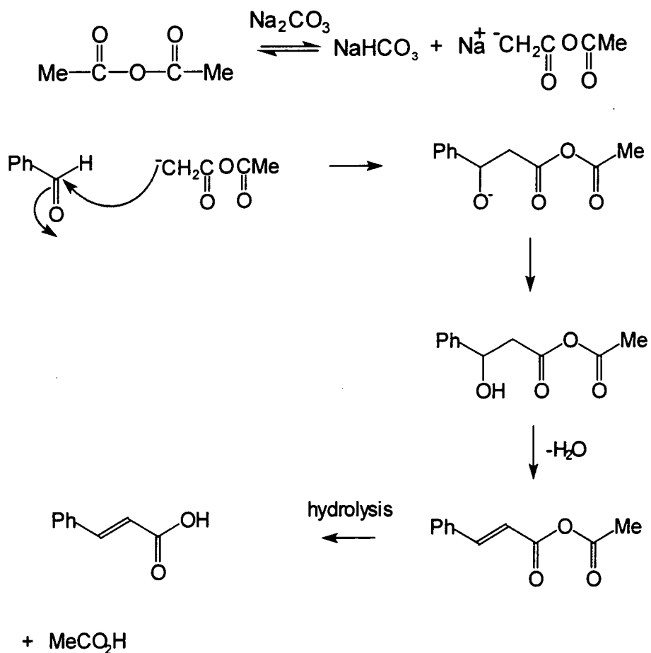
Figure 1.14 Perkin Reaction forming Cinnamic acid
