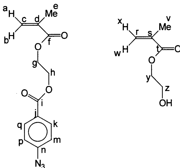
Figure 3.14 The Azide Monomer and HEMA in the Monomer Mixture
