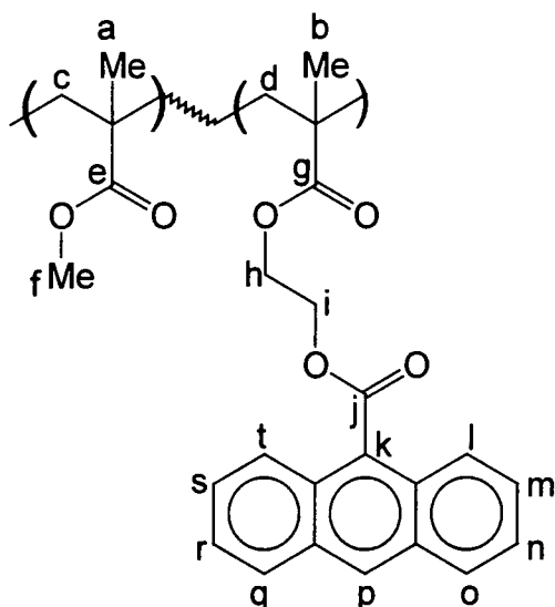
Figure 4.2 Poly(9'-anthracenoate-2-ethyl methacrylate-co-methyl methacrylate)
