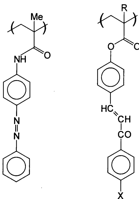
Figure 1.18 Examples of other Photosensitive Polymers
