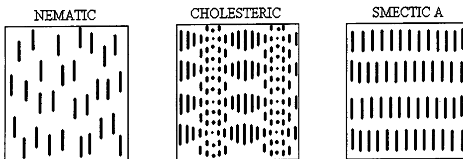
Figure 1.1 Types of Liquid Crystal
