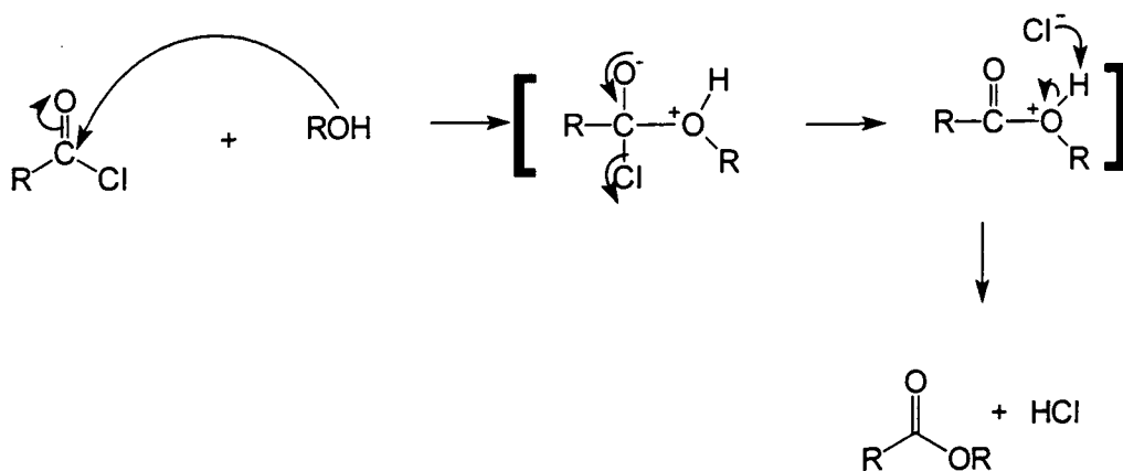
Figure 2.8 Ester formation mechanistic pathway
