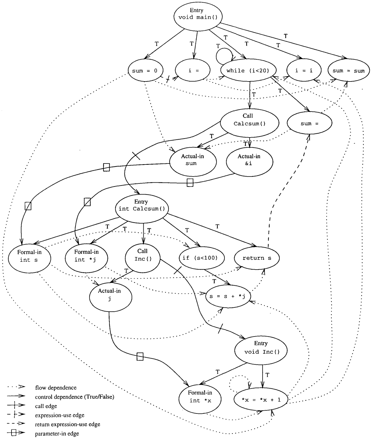
Figure 4.19: Example CCG.
