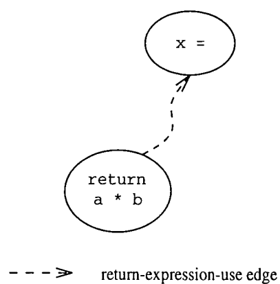
Figure 4.3: Return-expression-use edge.
