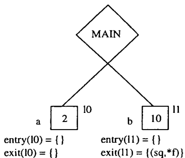
Figure 4.17: Data dependence analysis for example program cont.
