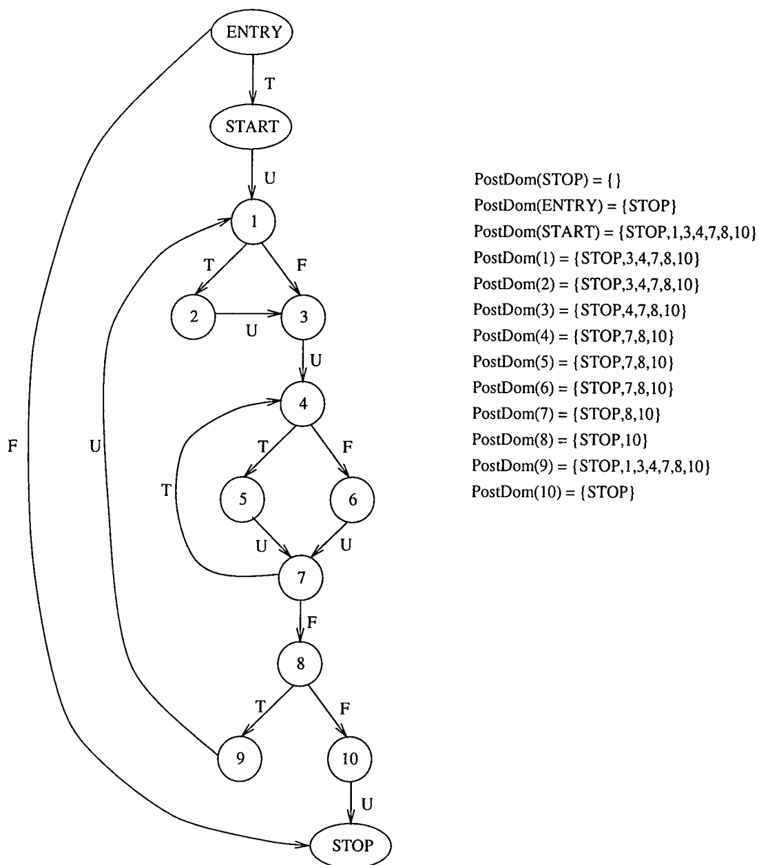
Figure 4.14: Control flow graph and post-dominator sets.
