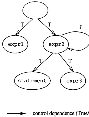
Figure 4.7: CCG control structure for for statement.
