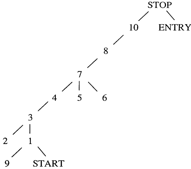
Figure 4.15: Post-dominator tree.
