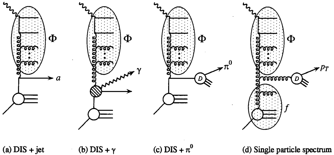
Figure 9.1: Diagrammatic representation of (a) the deep inelastic + forward jet, (b) the DIS + forward \gamma , (c) the DIS + forward \pi^0 , and (d) the single particle spectrum measurement.
