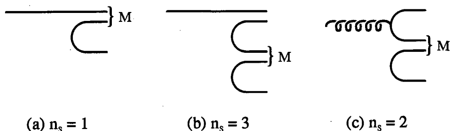
Figure 5.3: The minimum number of spectators, n_s , for fragmentation into a meson M for three different cases: fragmentation of a quark or antiquark which (a) is and (b) is not a constituent of M , and (c) fragmentation of a gluon [58].
