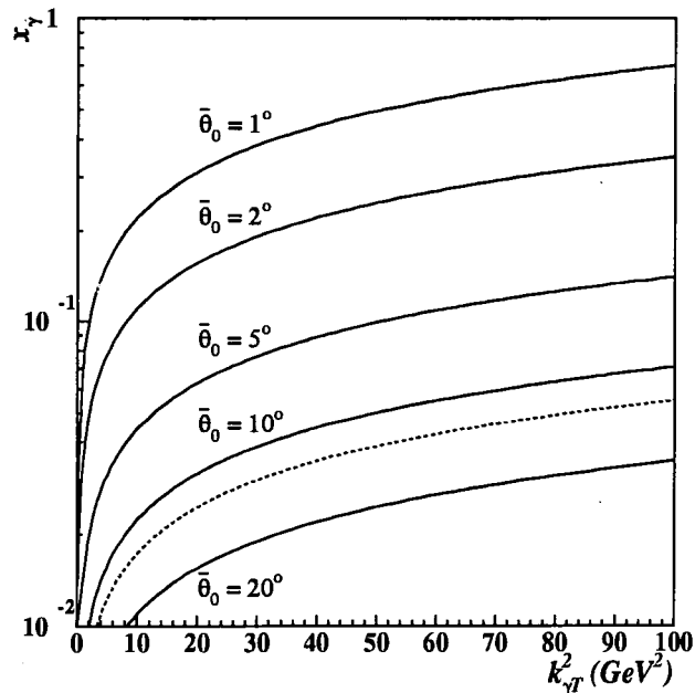
Figure 4.5: The curves give the upper boundary of the allowed regions of the photon kinematic variables (x_\gamma, k_{\gamma T}^2) for deep-inelastic + photon events with x = 6 \times 10^{-4} and Q^2 = 20 \text{ GeV}^2 for various choices of the acceptance angle \bar{\theta}_0 of (4.20). The photon angle \theta_{\gamma p} to the proton direction in the HERA ( 30 \times 820 \text{ GeV} ) laboratory frame is not uniquely specified by (x, Q^2; x_\gamma, k_{\gamma T}^2) . Varying the remaining azimuthal angle transforms the lines of constant \theta_{\gamma p} into narrow bands in the x_\gamma, k_{\gamma T}^2 plane. The continuous lines that are shown are obtained by averaging over the azimuthal degree of freedom. The lines are insensitive to reasonable variations of x and Q^2 . Also shown (by a dashed line) is the lower boundary given by the hemisphere cut (4.18) for x = 6 \times 10^{-4} and Q^2 = 20 \text{ GeV}^2 .
