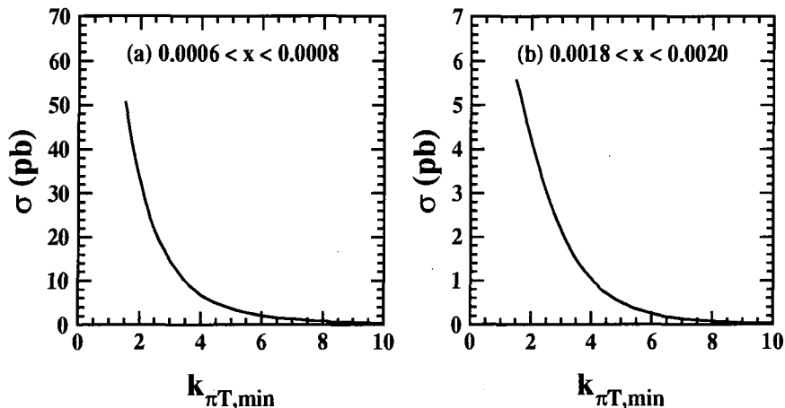
Figure 7.6: The DIS + \pi^0 cross section in the bins 20 < Q^2 < 30 \text{ GeV}^2 and (a) 6 \times 10^{-4} < x < 8 \times 10^{-4} and (b) 1.8 \times 10^{-3} < x < 2 \times 10^{-3} . The fragmentation scale and cuts are as for Fig. 7.4 but we vary the lower limit k_{\pi T, \min} on the transverse momentum of the \pi^0 .
