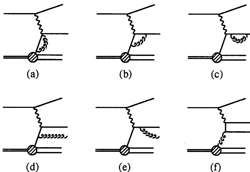
Figure 1.4: The \mathcal{O}(\alpha_S) contributions to deep inelastic ep scattering from (a) – (c) virtual gluons, (d) – (e) real gluons, and (f) a gluon inside the proton.
