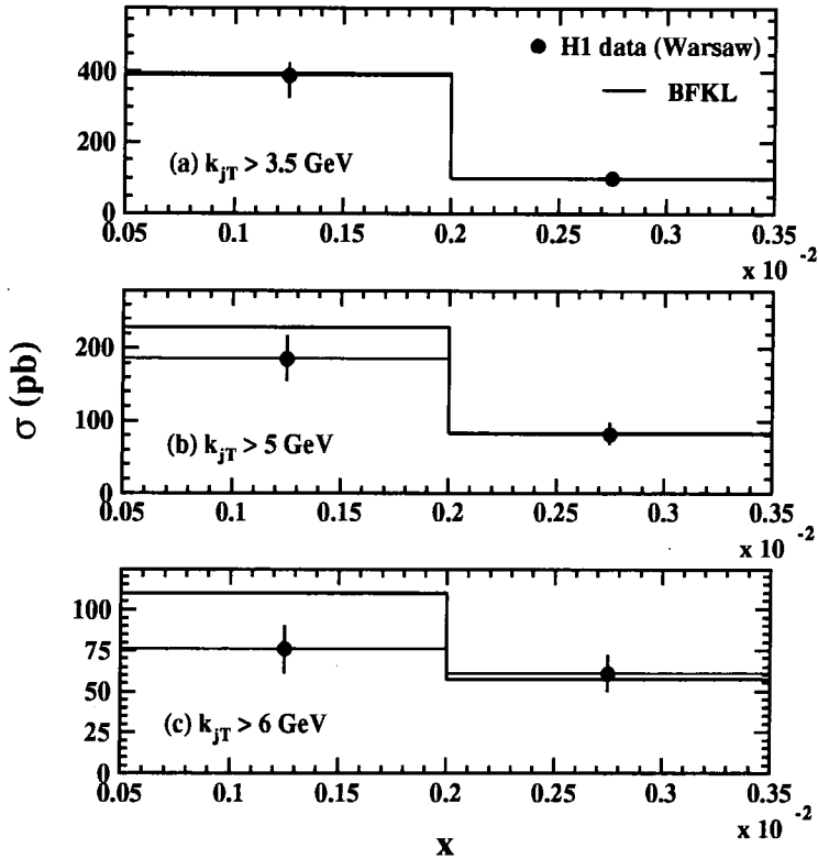
Figure 6.3: The deep inelastic + forward jet cross section in pb integrated over bins of size 1.5 \times 10^{-3} in x compared to the H1 data. Here z_0 = 0.15 and the cuts are the same as for Fig. 6.2 with exception of the minimum transverse momentum of the jet. The solid lines correspond to (a) k_{jT} > 3.5 GeV, (b) k_{jT} > 5 GeV and (c) k_{jT} > 6 GeV.
