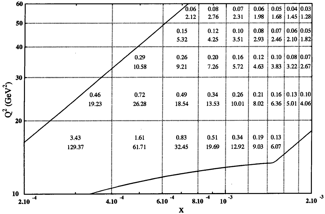
Figure 5.9: The upper and lower numbers are respectively the DIS + \pi^0 and DIS + jet cross sections (in pb) in various bins of x and Q^2 . For the pion the cuts are those given in Fig. 5.7, and exactly the same cuts are used for the forward jet.
