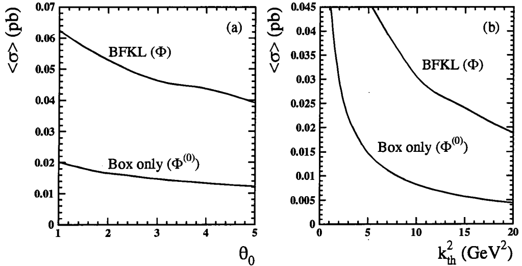
Figure 4.6: The dependence of the DIS + \gamma cross section integrated over the photon variables to variation of (a) the angle \theta_0 defining the isolation cone around the photon ( \theta_{\gamma j} > \theta_0 ) and (b) the threshold for photon detection ( k_{\gamma T}^2 > k_{th}^2 ). The results are for the x, Q^2 bin defined by 6 \times 10^{-4} < x < 8 \times 10^{-4} and 20 < Q^2 < 30 \text{ GeV}^2 . We impose the hemisphere cut (4.19) and take \bar{\theta}_0 = 5^\circ in (4.20). (The lack of smoothness of the curves simply reflects the errors on the six-fold numerical integration).
