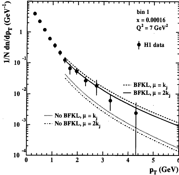
Figure 8.4: The transverse momentum spectrum of charged particles ( \pi^+ , \pi^- , K^+ , K^- ) in the pseudo-rapidity interval 0.5 < \eta < 1.5 in the virtual photon-proton centre-of-mass frame. The results are shown for kinematic bin 1 with the central values x = 1.6 \times 10^{-4} and Q^2 = 7 \text{ GeV}^2 . The continuous and the dashed curve show the spectra obtained with \Phi_i and f calculated from the BFKL equation. They only differ in the choice of fragmentation scale: for the continuous curve the fragmentation functions were evaluated at scale \mu^2 = (2k_j)^2 and for the dashed curve at scale \mu^2 = k_j^2 . When BFKL radiation is neglected in the calculation of the p_T spectra, i.e. when the quark box approximation \Phi_i = \Phi_i^{(0)} is used and strong ordering at the gluon vertex is assumed, then the dash-dotted and dotted curves are obtained. The fragmentation functions were evaluated at scales \mu^2 = (2k_j) and k_j^2 respectively. The data points shown are from the H1 measurement of the charged particle spectra [71].
