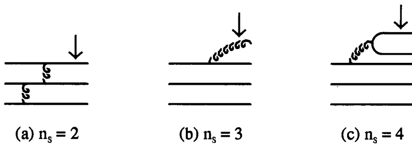
Figure 1.3: The minimum number of spectators, n_s , for (a) a valence quark, (b) a gluon, and (c) a sea quark. The parton under consideration is marked by an arrow.
