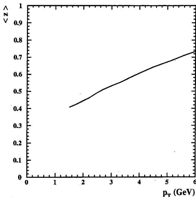
Figure 8.9: The average value of the fraction z of the parton jet's momentum which the emitted hadron carries away versus the transverse momentum p_T of the hadron.
