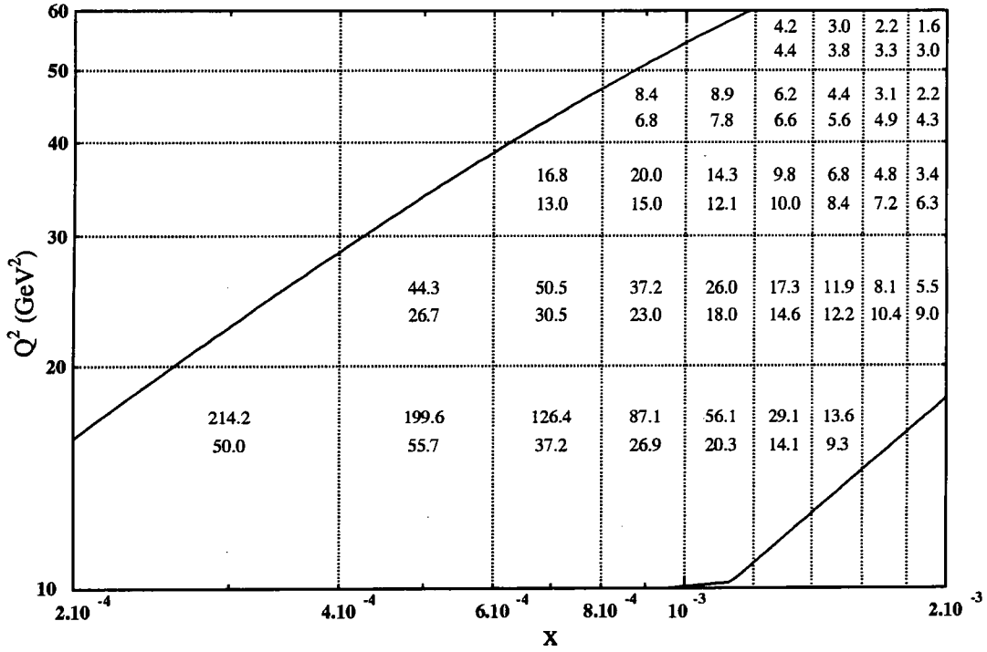
Figure 7.10: The upper and lower numbers correspond to the DIS + \pi^0 and the DIS + jet cross sections in pb, respectively. The results are shown in bins in x and Q^2 which are accessible at HERA. The DIS + \pi^0 cross section was calculated as for Fig. 7.5 and the DIS + jet cross section was obtained as for Fig. 7.1 but subject to the same electron acceptance region as the \pi^0 which is given in (7.1).
