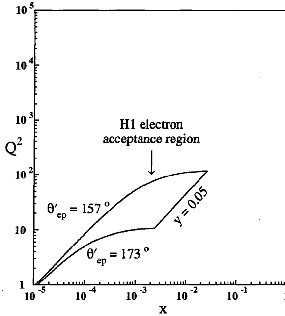
Figure 8.3: The acceptance region for the scattered electron specified by 0.05 < y < 1 and 157^\circ < \theta'_{ep} < 173^\circ in the HERA laboratory frame.
