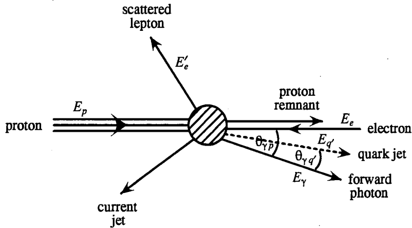
Figure 4.4: Kinematics of the deep inelastic + forward photon process.
