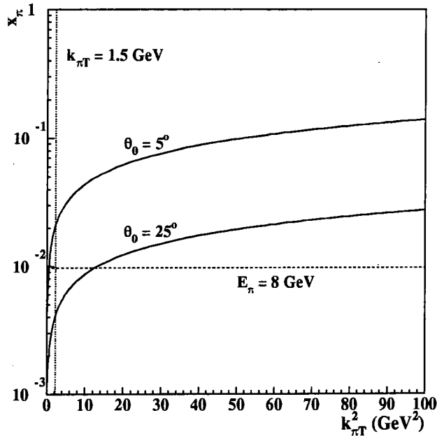
Figure 7.3: The accessible (x_\pi, k_{\pi T}^2) region defined by the cuts given in (7.3) – (7.5). The curves corresponding to \theta_{\pi p} = \theta_0 = 25^\circ (solid line) and E_\pi = 8 GeV (dashed line) represent the lower boundaries, whereas the solid curve for \theta_0 = 5^\circ describes the upper boundary. Also shown, as a dotted line, is the boundary defined by k_{\pi T} > 1.5 GeV. Note that the solid lines were calculated as for Fig. 5.5.
