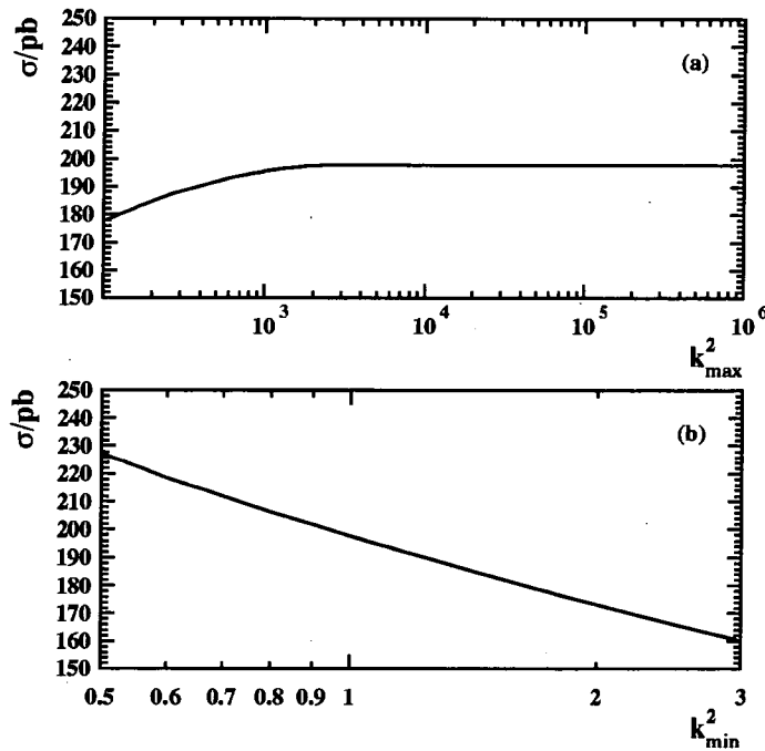
Figure 6.4: The dependence of the deep inelastic + forward jet cross section in pb in the bin 5 \times 10^{-4} < x < 10^{-3} on (a) the upper limit k_{\text{max}}^2 and (b) the lower limit k_{\text{min}}^2 on the transverse momentum integration in the BFKL equations. The cuts are the same as for Fig. 6.2 and z_0 = 0.15 .
