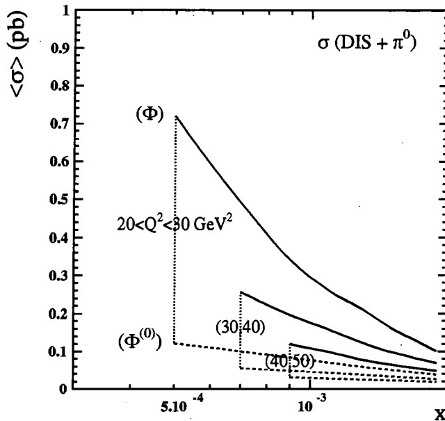
Figure 5.6: The cross section, \langle\sigma\rangle in pb, for deep inelastic + \pi^0 events integrated over bins of size \Delta x = 2 \times 10^{-4} , \Delta Q^2 = 10 \text{ GeV}^2 which are accessible at HERA for \pi^0 's with transverse momentum 3 < k_{\pi T} < 10 \text{ GeV} where the constraints x_\pi > 0.05 , \theta_{\pi p} > 5^\circ , and the hemisphere cut, (5.28), were imposed. The fragmentation functions were evaluated at scale k_{\pi T}^2 . The \langle\sigma\rangle values are plotted at the central x value in each \Delta x bin and joined by straight lines. The x dependence is plotted for three different \Delta Q^2 bins, namely (20,30), (30,40) and (40,50) \text{GeV}^2 . The continuous curves show \langle\sigma\rangle calculated with \Phi_i obtained from the BFKL equation. The corresponding \langle\sigma\rangle values calculated neglecting soft gluon resummation and just using the quark box approximation \Phi_i = \Phi_i^{(0)} are plotted as dashed curves. For clarity a dotted vertical line joins each pair of curves belonging to the same \Delta Q^2 bin.
