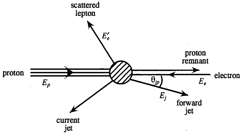
Figure 3.9: Kinematics of the DIS + jet process.
