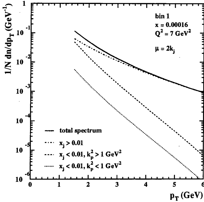
Figure 8.7: Contributions to the single particle spectrum in kinematic bin 1 with the central values x = 1.6 \times 10^{-4} and Q^2 = 7 \text{ GeV}^2 . Shown as a solid line is the total spectrum calculated as for Fig. 8.4 including BFKL resummation in the calculation and evaluating the fragmentation functions at scale \mu^2 = (2k_j)^2 . Dash-dotted and dotted lines represent the contributions from the regions x_j > 10^{-2} and x_j < 10^{-2} , k_p^2 < 1 \text{ GeV}^2 , respectively. In these cases only one BFKL ladder, \Phi , is included. Two BFKL ladders, \Phi and f , contribute to the differential structure functions – and therefore the p_T spectrum – in the region x_j < 10^{-2} , k_p^2 > 1 \text{ GeV}^2 , as is displayed as a dashed line.
