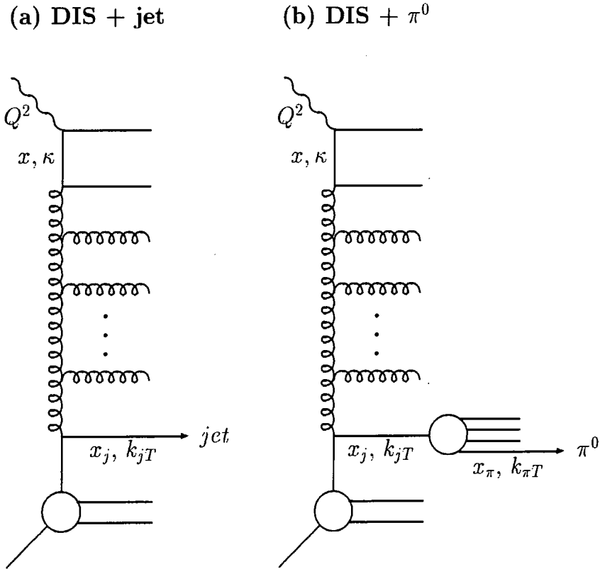
Figure 5.1: Diagrammatic representation of (a) a deep inelastic + forward jet event, and (b) a deep inelastic (x, Q^2) + identified forward \pi^0 (x_\pi, k_{\pi T}) event.
