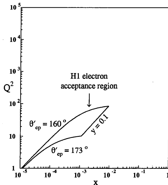
Figure 6.1: The acceptance region in the (x, Q^2) plane for deep inelastic events defined by 160^\circ < \theta'_{ep} < 173^\circ and 0.1 < y < 1 in the HERA ( 27.5 \times 820 GeV) laboratory frame.
