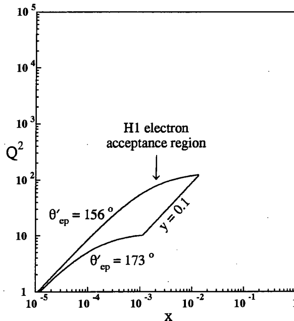
Figure 7.2: The acceptance region for the outgoing lepton defined by 0.1 < y < 1 and 156^\circ < \theta'_{ep} < 173^\circ in the HERA ( 27.5 \times 820 GeV) laboratory frame.
