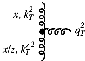
Figure 2.8: Fragment of (the left half of) a BFKL ladder diagram. x and x/z are the fractions of the proton's longitudinal momentum carried by the gluons. The transverse momenta of the gluons along the ladder and of the emitted gluon are denoted by k_T , k_T' and q_T , respectively.
