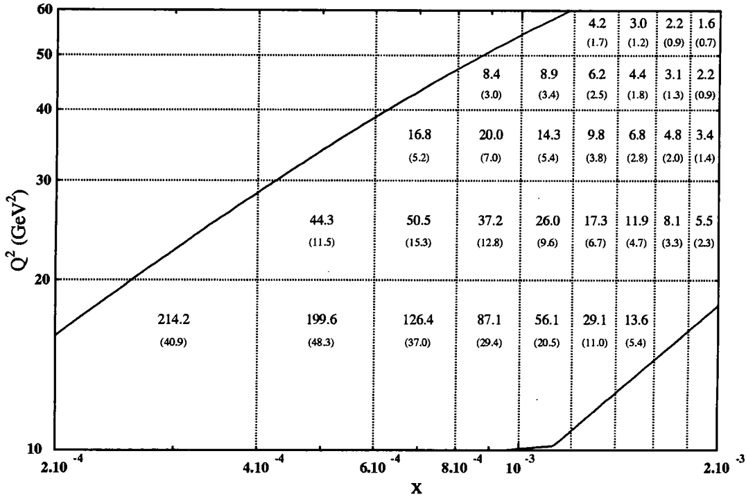
Figure 7.5: The DIS + \pi^0 cross section \langle\sigma\rangle in pb in bins in x and Q^2 which are accessible at HERA. As for Fig. 7.4 the outgoing lepton was required to fulfil (7.1) and the \pi^0 (7.3) – (7.6). Again the fragmentation functions were evaluated at scale \mu^2 = k_{\pi T}^2 . The values in brackets correspond to \langle\sigma\rangle computed using the quark box approximation \Phi_i = \Phi_i^{(0)} . Shown as continuous lines are the boundaries on the acceptance region at HERA defined by 156^\circ < \theta'_{ep} < 173^\circ and y > 0.1 .
