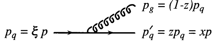
Figure 1.6: A quark of momentum p_q = \xi p emits a gluon and remains with momentum p'_q = xp where p is the momentum of the proton. Then the final quark carries a fraction z = x/\xi of the parent quark's momentum.
