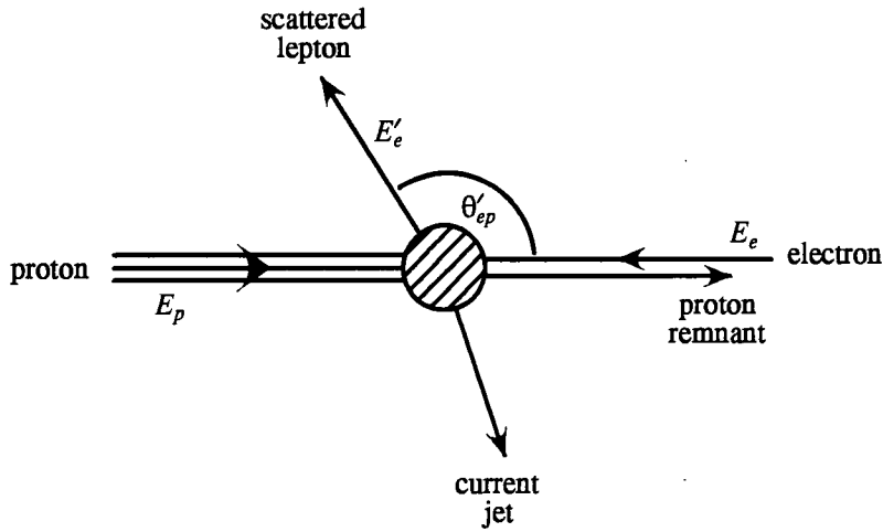
Figure 3.7: Kinematics of a deep inelastic event.
