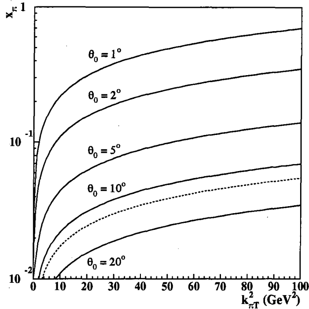
Figure 5.5: The relation between the \pi^0 kinematic variables for DIS + \pi^0 events with x = 6 \times 10^{-4} and Q^2 = 20 \text{ GeV}^2 for various choices of the angle \theta_0 in (5.31). In the HERA ( 27.6 \times 820 \text{ GeV} ) laboratory frame the pion angle \theta_{\pi p} to the proton direction is not uniquely specified by (x, Q^2; x_\pi, k_{\pi T}^2) . Varying the remaining azimuthal angle transforms the lines of constant \theta_{\pi p} into narrow bands in the x_\pi, k_{\pi T}^2 plane. Here we averaged over the azimuthal degree of freedom. The plot is insensitive to variations of x, Q^2 over their relevant intervals. The continuous lines are the upper boundary on the allowed kinematic region for different choices of \theta_0 . The dashed line represents the lower boundary given by the hemisphere cut, (5.28), for x = 6 \times 10^{-4} and Q^2 = 20 \text{ GeV}^2 .
