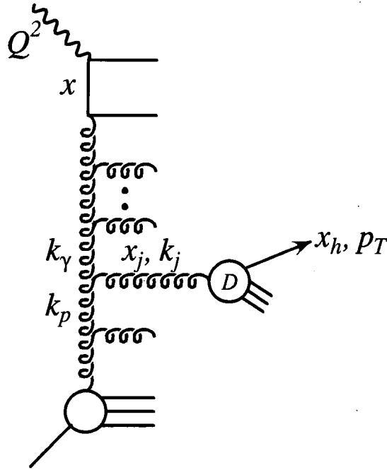
Figure 8.2: Diagrammatic representation of the cross section for emission of a high transverse momentum p_T particle.
