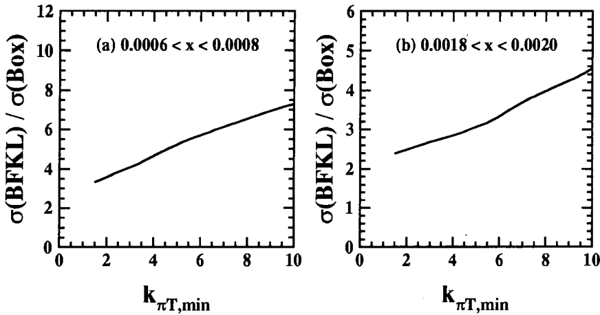
Figure 7.7: The ratio of the DIS + \pi^0 cross section calculated as for Fig. 7.6 and the cross section obtained when using the quark box approximation \Phi = \Phi^{(0)} . The results are shown for the bins defined by 20 < Q^2 < 30 \text{ GeV}^2 and (a) 6 \times 10^{-4} < x < 8 \times 10^{-4} and (b) 1.8 \times 10^{-3} < x < 2 \times 10^{-3} .
