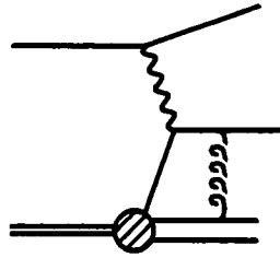
Figure 1.5: A higher twist contribution to deep inelastic ep scattering.
