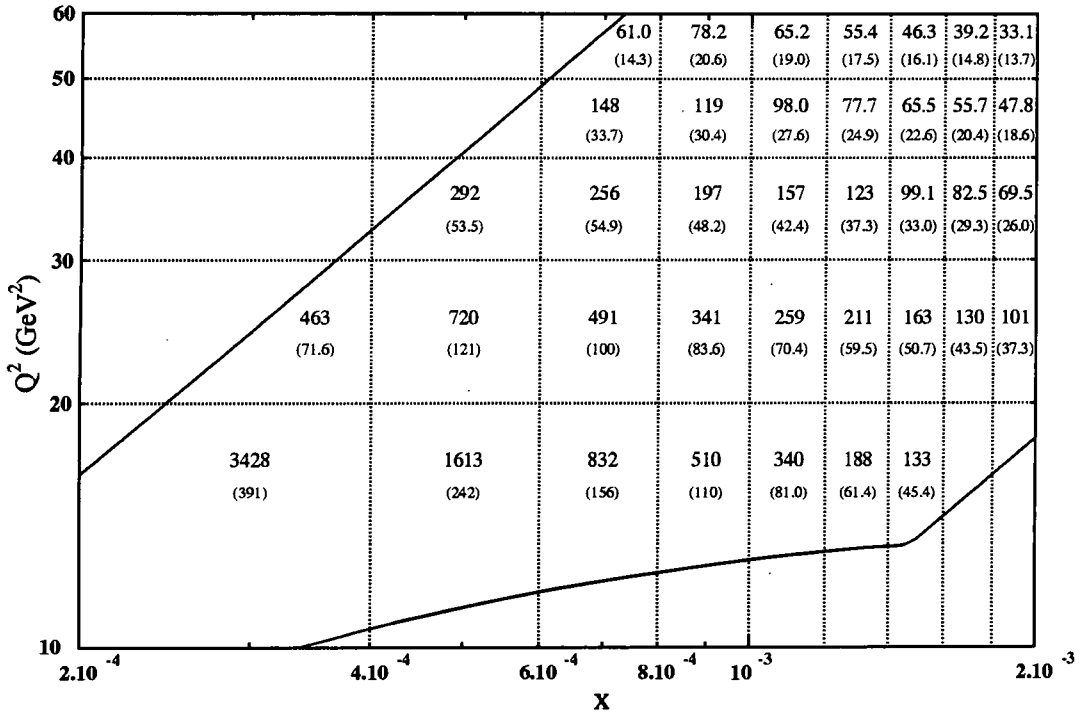
Figure 5.7: The cross section, \langle\sigma\rangle in fb, for deep inelastic + \pi^0 events in various (\Delta x, \Delta Q^2) bins which are accessible at HERA, and integrated over the region 3 < k_{\pi T} < 10 GeV, \theta_{\pi p} > 5^\circ , x_\pi > 0.05 , and subject to the hemisphere cut, (5.28). The fragmentation functions were evaluated at scale \mu^2 = k_{\pi T}^2 . The values in brackets are the cross sections obtained when using only the quark box approximation \Phi_i = \Phi_i^{(0)} . Therefore the difference between the two numbers shown in one bin is the enhancement due to BFKL soft gluon resummation. Recall that (5.20) implies that the results shown for the DIS + \pi^0 cross section here equal the average of the cross sections for \pi^+ and \pi^- production. The curves are the boundaries of the acceptance regions at HERA given by 8^\circ < \theta'_{ep} < 172^\circ and 0.1 < y < 0.9 .
