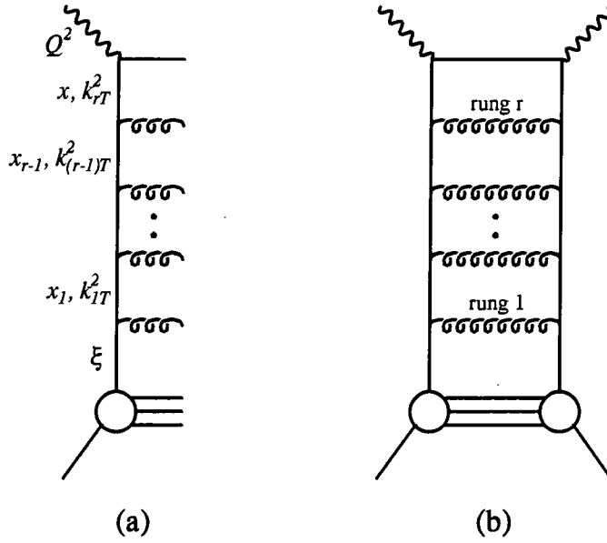
Figure 2.1: Diagrammatic representation of probing the proton at large x with a photon of large virtuality Q^2 . Squaring the amplitude shown in (a) produces the ladder diagram in (b). The DGLAP equations sums the leading terms in \ln Q^2 which are generated by ladder diagrams of this form with the transverse momenta ( k_{iT} ) strongly ordered and the longitudinal momenta ( x_i p ) ordered.
