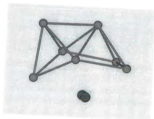
Figure 4.23: \text{Ar}_7\text{N}_2 V_{7,3} structure
