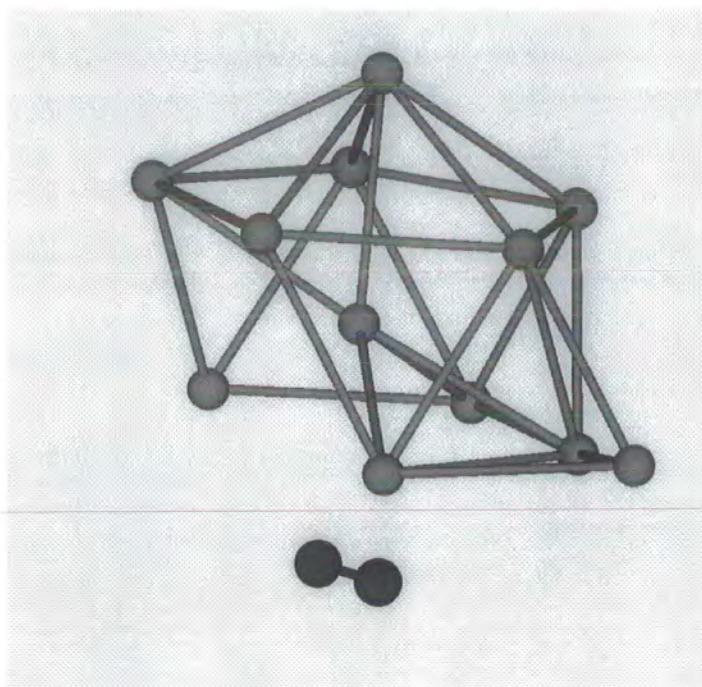
Figure 4.49: \text{Ar}_{12}\text{N}_2 V_{12,6} structure
