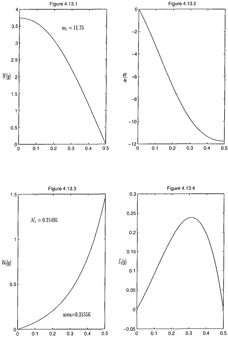
Figure 4.13: The eigen-state of j = 1 for the charged interior of a Schwarzschild black hole with parameters, q = 0 , \epsilon_A = \epsilon_\theta = 1 , M = M_l , e = 10^{-3} .
