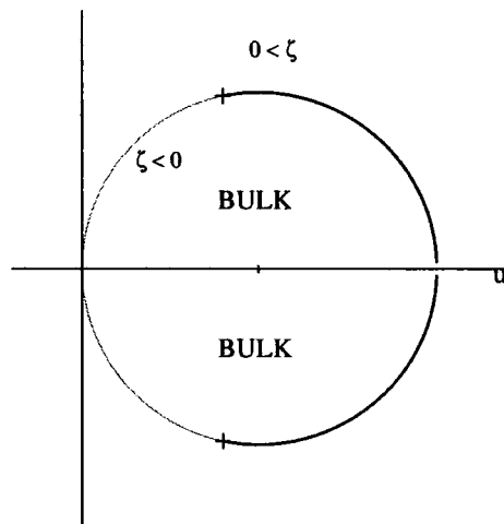
(c) Critical brane
