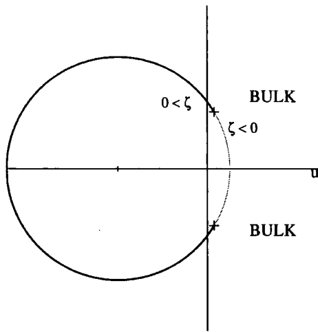
(a) Subcritical brane centered on -u_0
