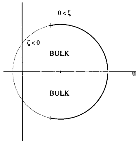
(b) Subcritical brane centered on +u_0
