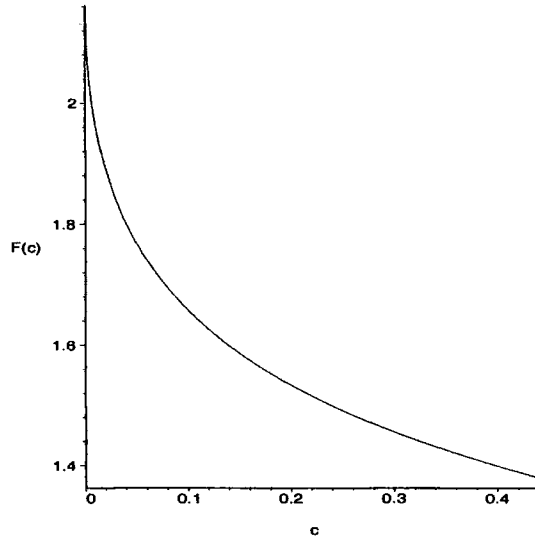
Figure 4.9: A plot of \mathcal{F}(c) for 0 \leq c \leq 1/4a when \tilde{\sigma} = 1.25 and k = 1 . Note that there is no solution to \mathcal{F}(c) = 0 .
