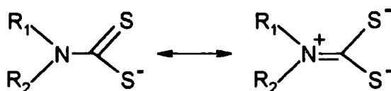
Figure 5.1 Structure and resonance forms of the dithiocarbamate functional group.
