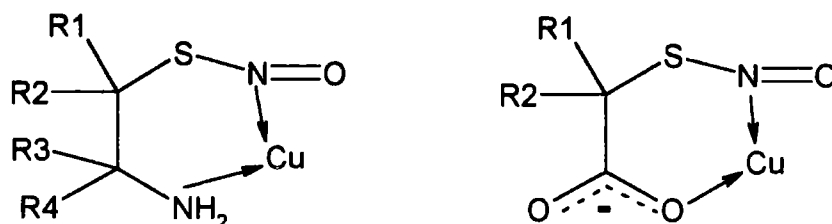
Figure 1.7 Suggested S -nitrosothiol copper reaction intermediates.
