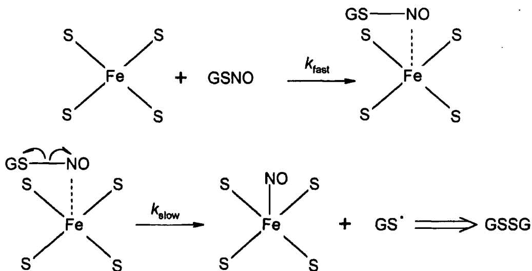
Scheme 5.11 Proposed mechanism for nitrosyl iron(+2) MGD complex formation using GSNO. (the dotted line represents atom interactions)
