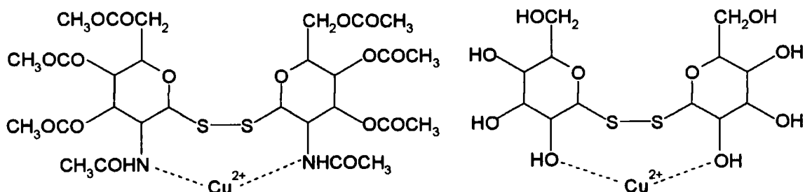
Figure 2.10 Proposed copper(+2) ion complexes with the disulfides of the S -nitroso sugars.
