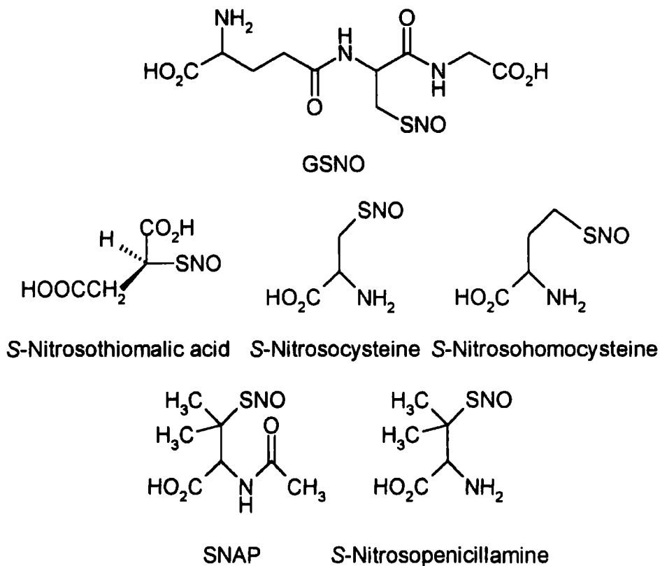
Figure 1.6 Structure and names of some S -nitrosothiols.
