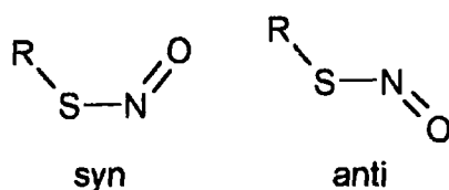
Figure 1.4 The structures of the syn and anti conformations of S -nitrosothiols.
