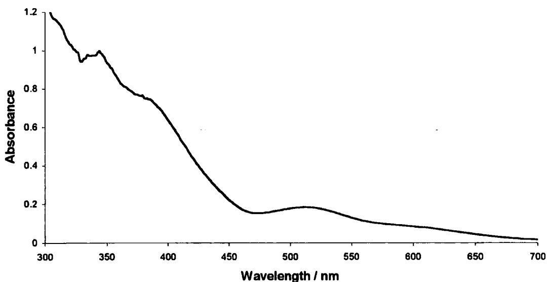
Figure 5.5 UV / Vis spectrum of a solution containing 1 \times 10^{-4} M \text{FeCl}_3 and 3 \times 10^{-4} M MGD.
