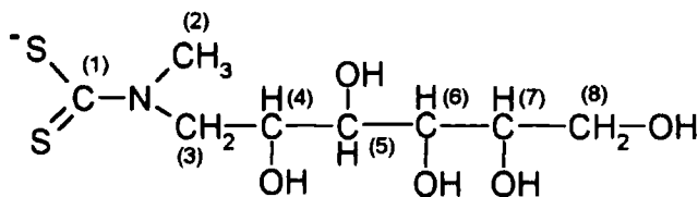
Figure 6.3 Structure of MGD.
