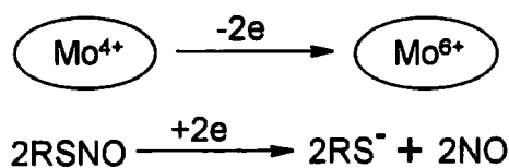
Scheme 1.31 Proposed mechanism for the superoxide independent decomposition of S -nitrosocysteine by xanthine oxidase.
