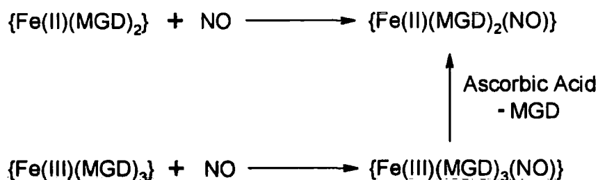
Scheme 5.2 Proposed reactions of NO with the iron MGD complexes.
