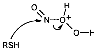
Scheme 1.8: Proposed mechanism for S -nitrosothiol formation from thiol and peroxyntrous acid.
