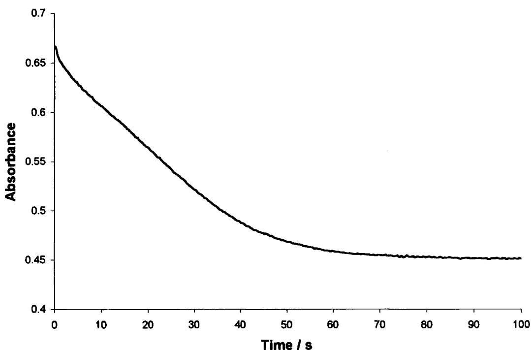
Figure 5.13 Absorbance at 511 nm measured over time for a solution containing 1 \times 10^{-2} M GSNO, 5 \times 10^{-4} M \{\text{Fe(III)}(\text{MGD})_3\} and 0.15 M TRIS buffer (pH 7.4).
