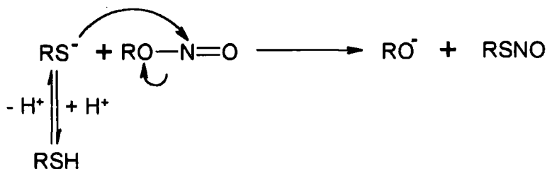
Scheme 1.9 Mechanism for the reactions of thiol with alkyl nitrites.
