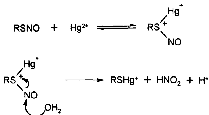
Scheme 1.18 Proposed mechanism for the mercury(+2) ion reaction with S -nitrosothiols.
