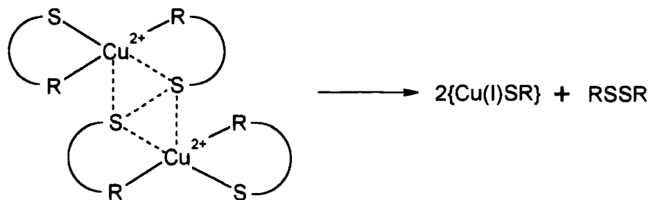
Scheme 1.15 Proposed mechanism for the reduction of copper(+2) by thiol.
