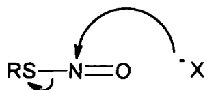
Scheme 1.19 General mechanism for the reaction of S -nitrosothiols with nucleophiles.
