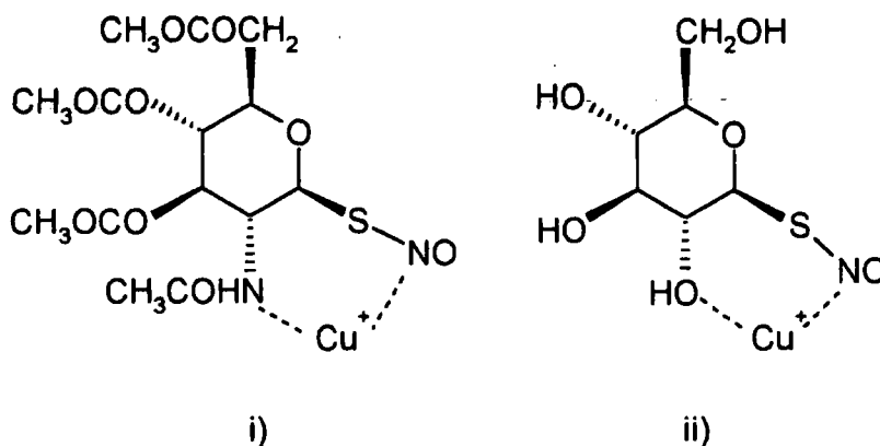
Figure 2.9 Proposed copper(+1) intermediates with i) GPSNO and ii) SNTG.
