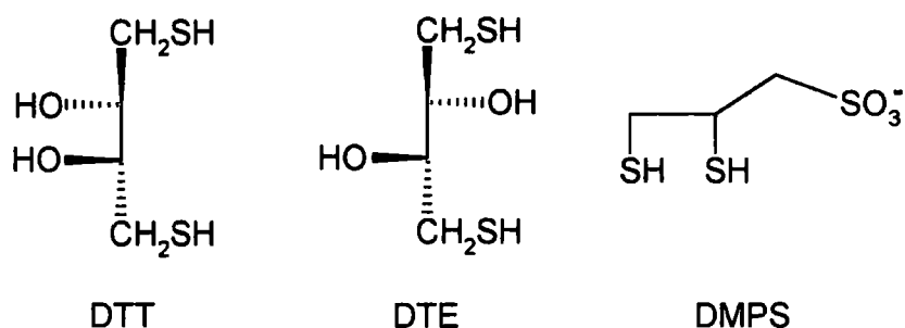
Figure 3.1 The structure of three dithiols.
