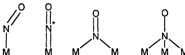
Figure 1.2 The possible coordination modes of NO in metal complexes.
