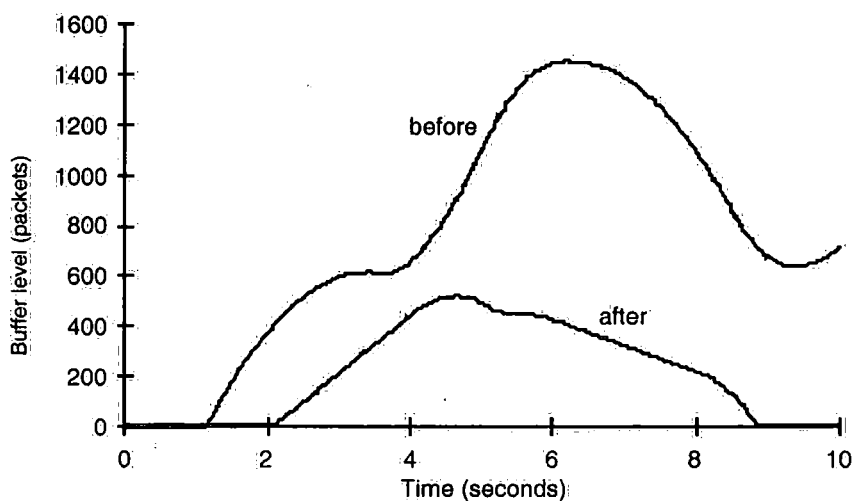
(e) Buffer level at end system J before and after reconfiguration
