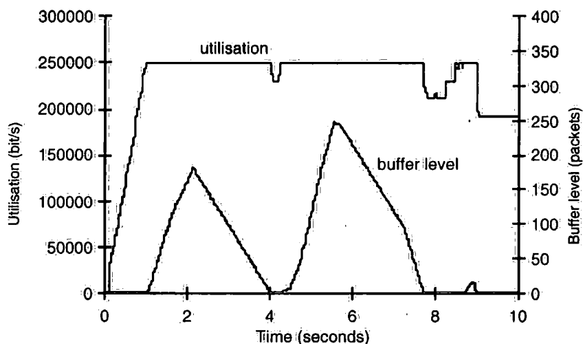
(d) Resource utilization and buffer level at <37-31> after reconfiguration
