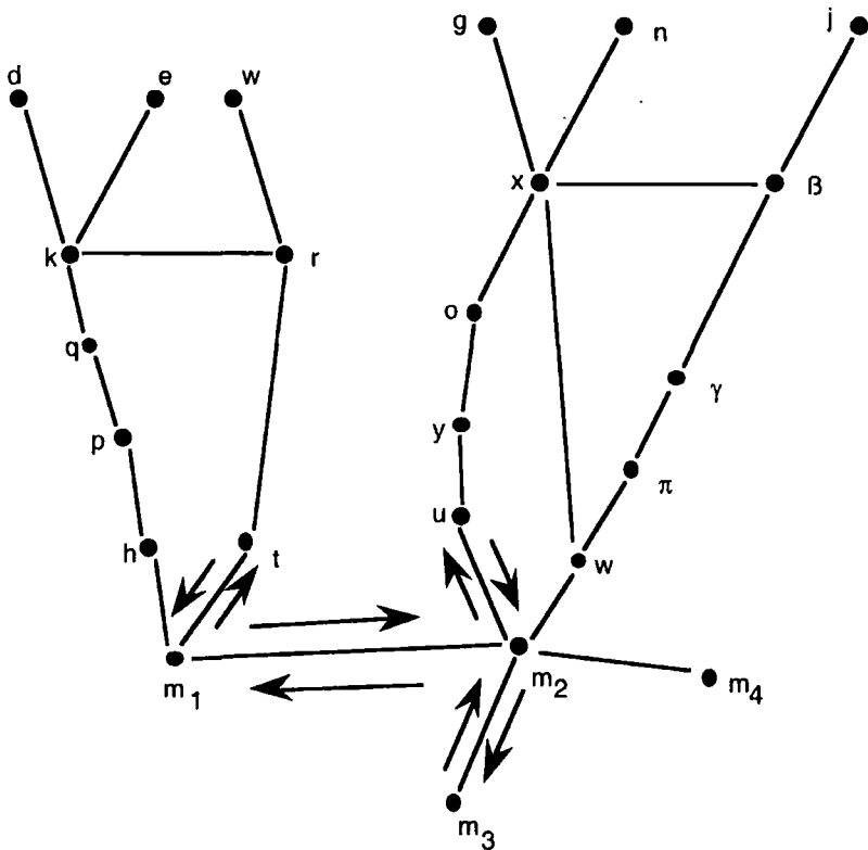
Figure 4.3 The structure of channels across end-systems
